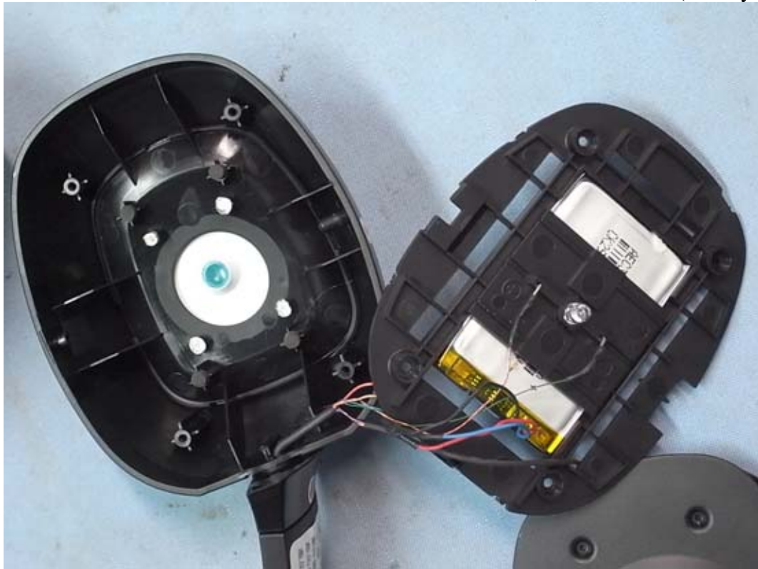
Figure 17 Left Headset, Internal View (Battery View)
