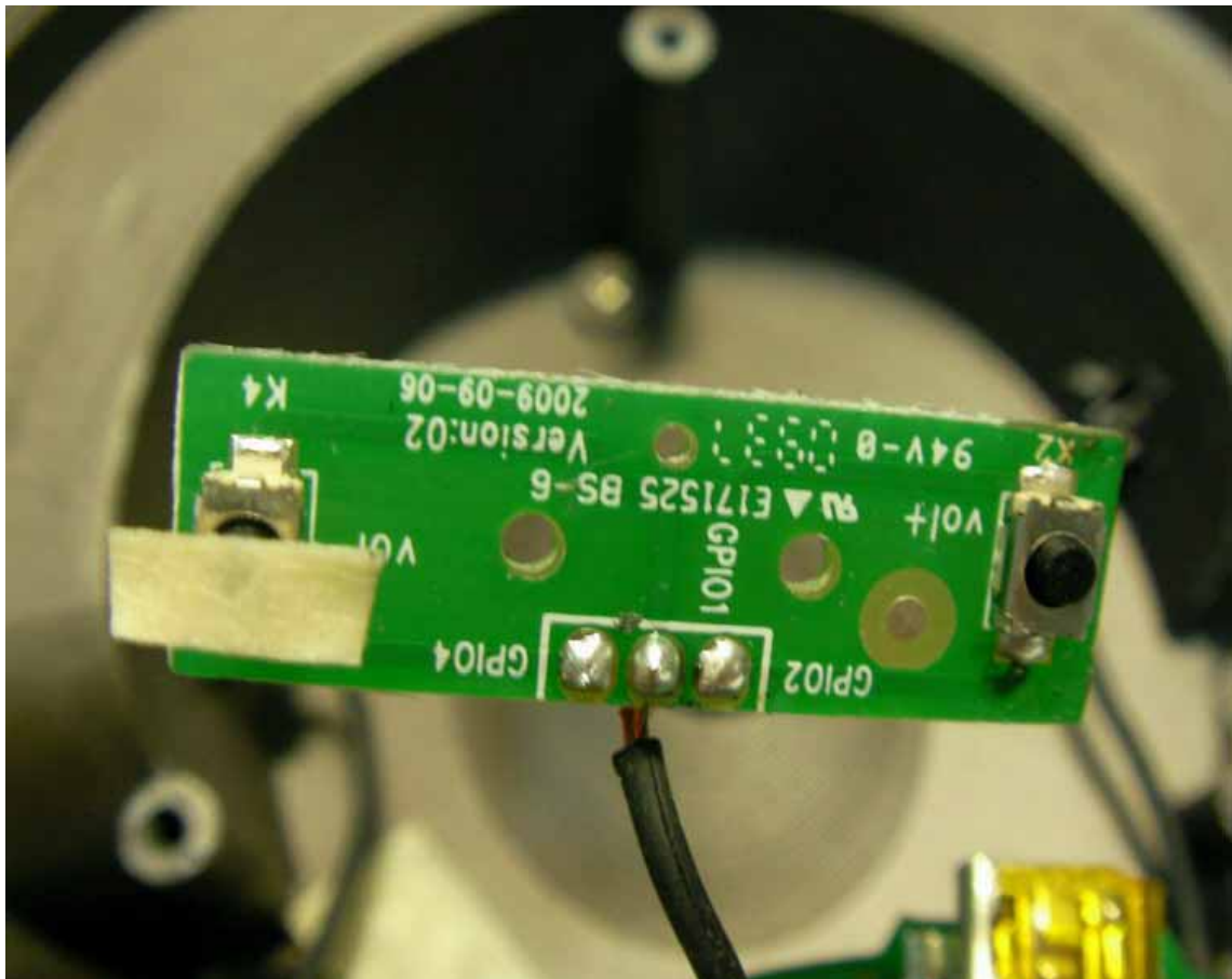
Figure 8 Inside of the EUT
