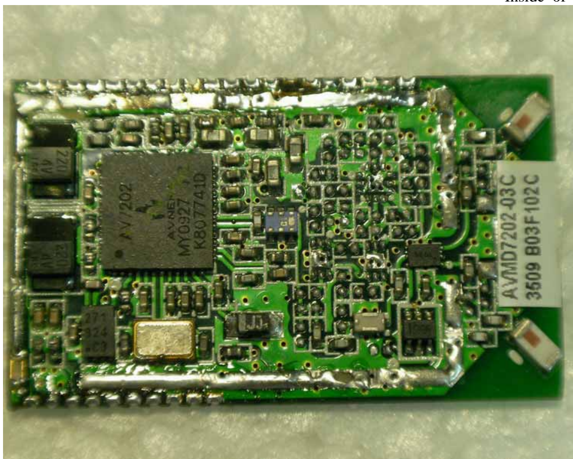
Figure 12 Inside of the EUT
