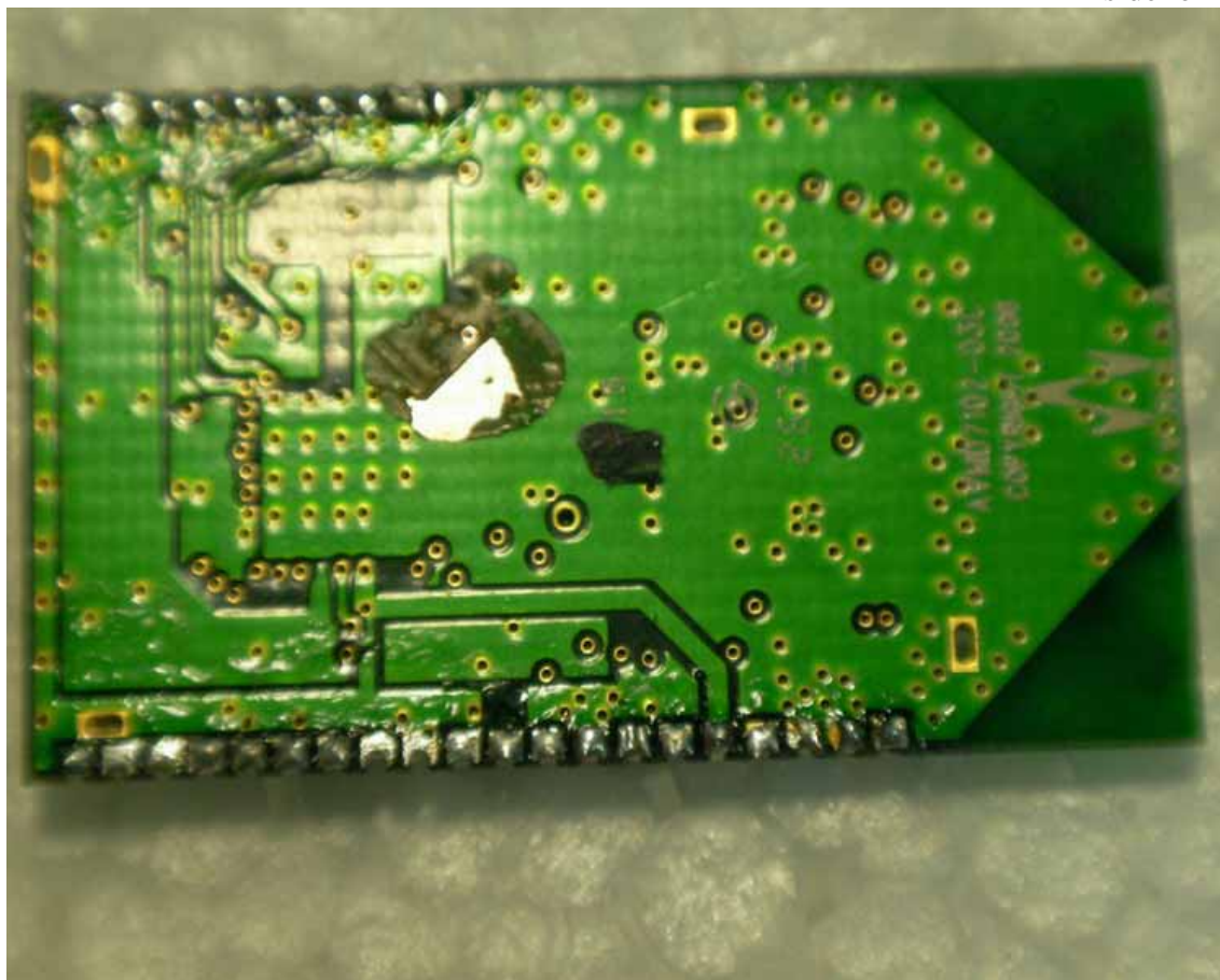
Figure 11 Inside of the EUT
