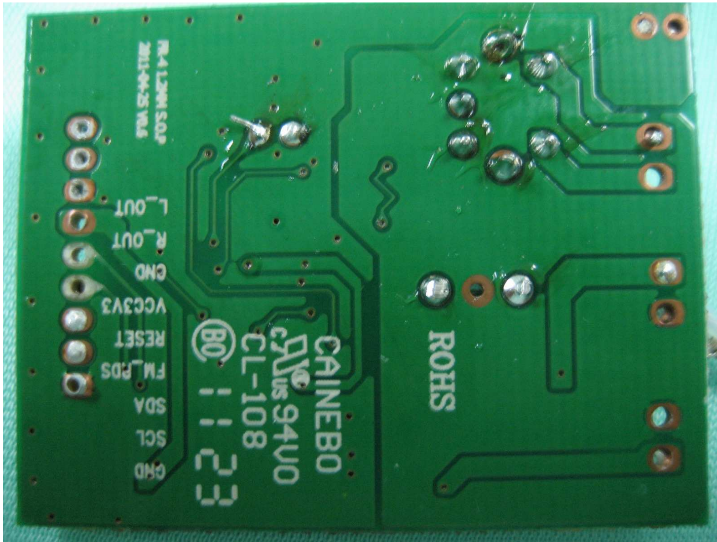
Rear View of the PCB – Tuner Part
