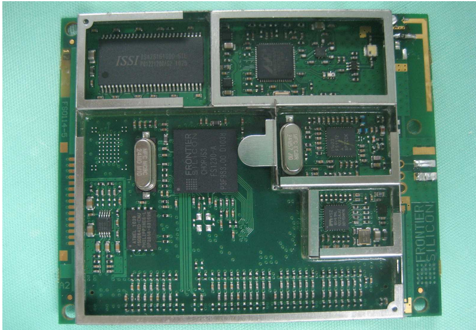
Front View of the PCB – V8 module
