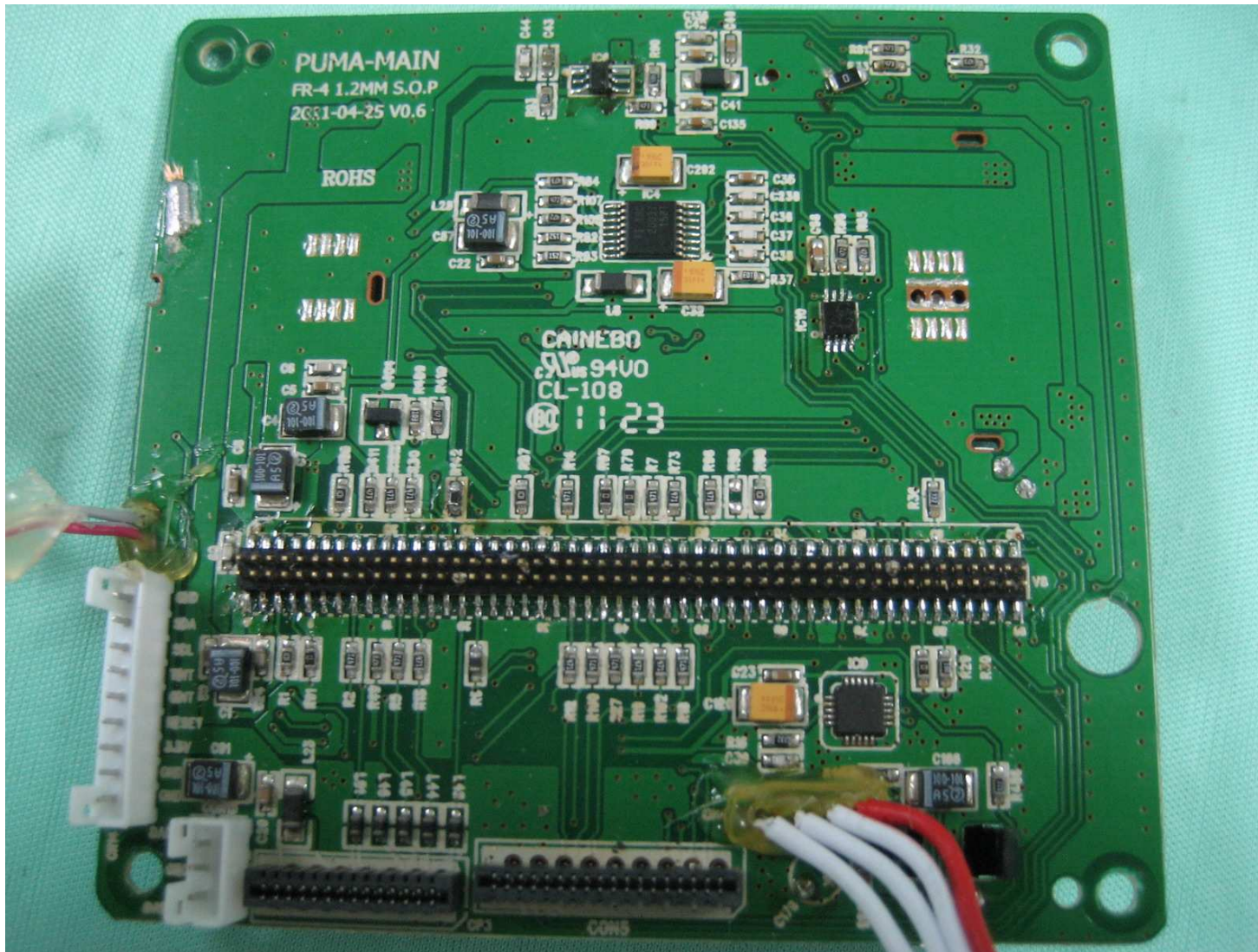
Rear View of the PCB – PUMA-MAIN
