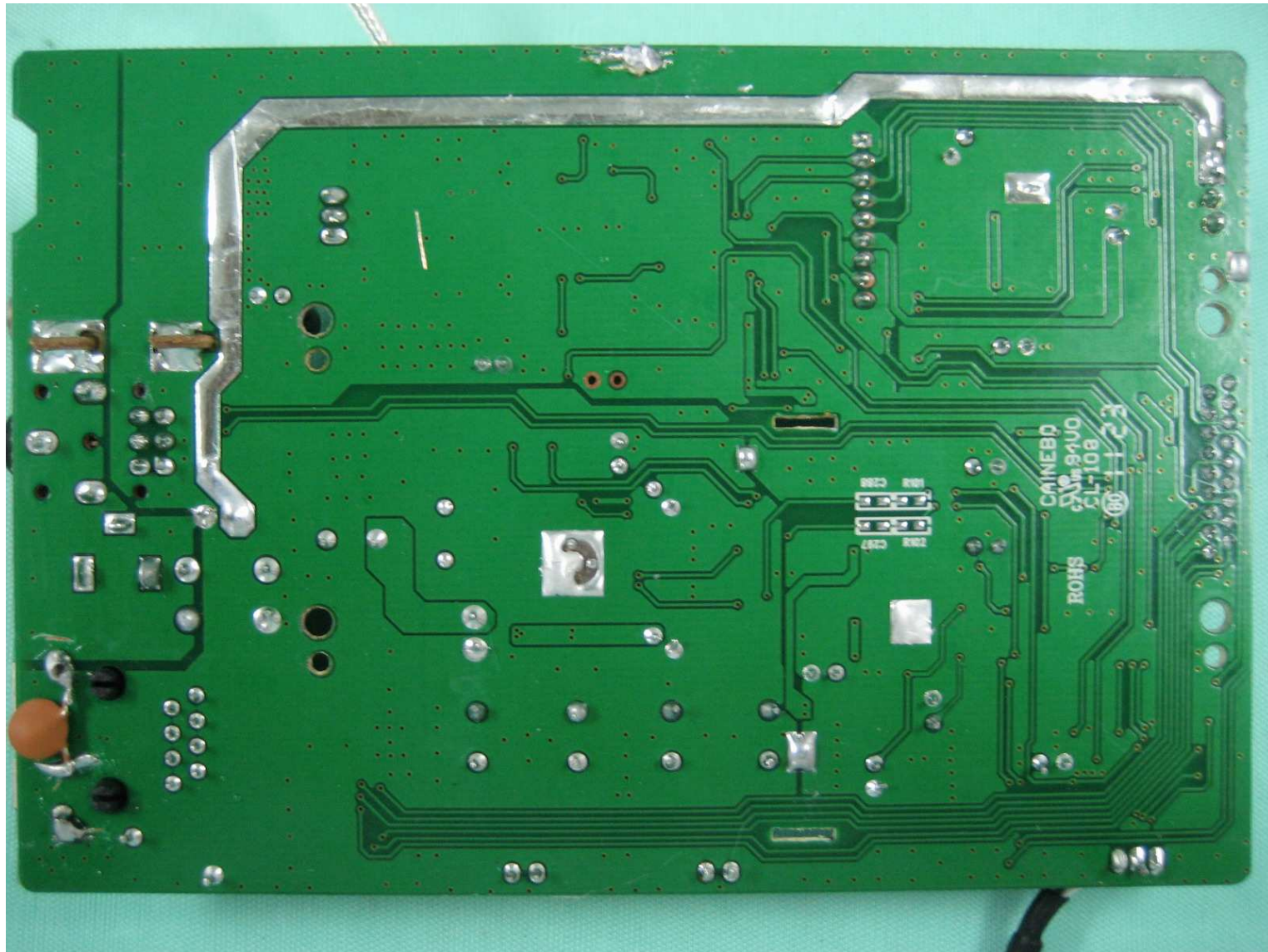
Rear View of the PCB – PUMA-POWER
