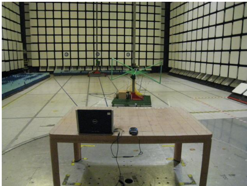
Transmitter Radiated Emissions Test Setup (Rear View)
