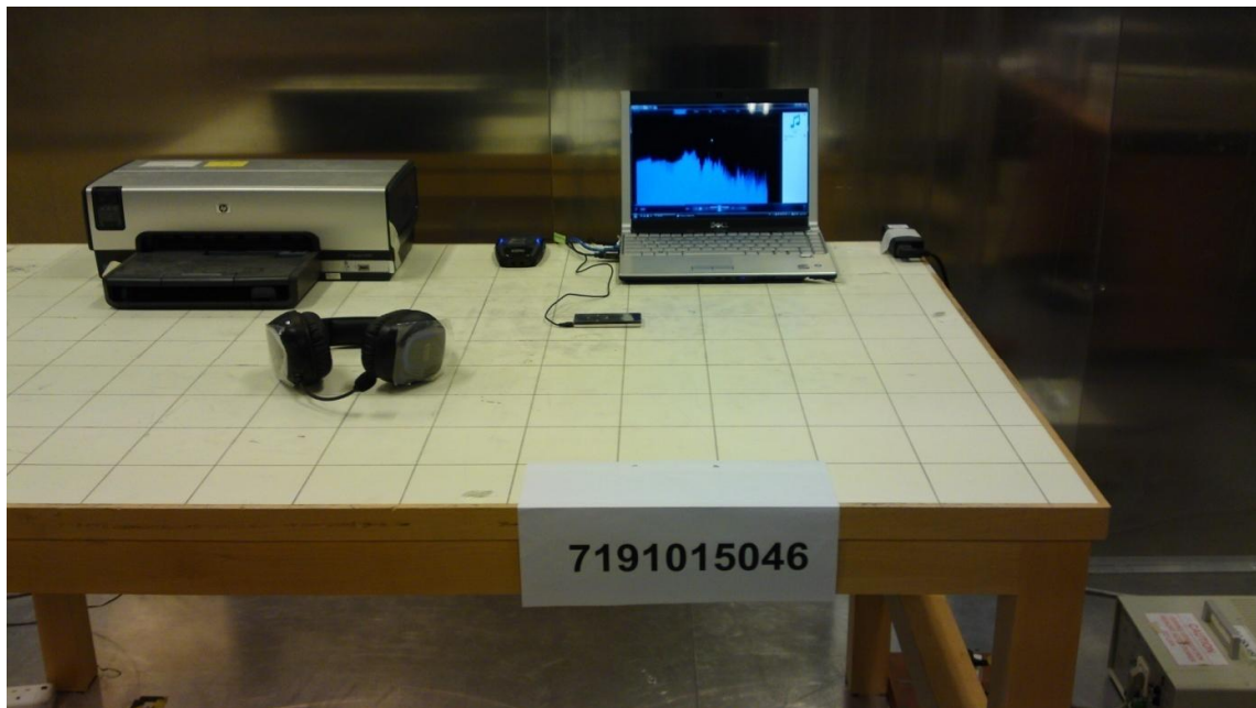
Conducted Emissions Test Setup (Front View)
