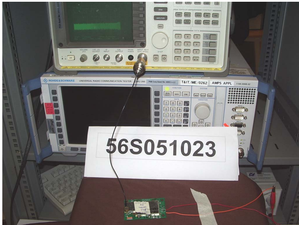
Spectrum Bandwidth (20dB Bandwidth Measurement) Test Setup NUMBER OF HOPPING FREQUENCIES TEST
