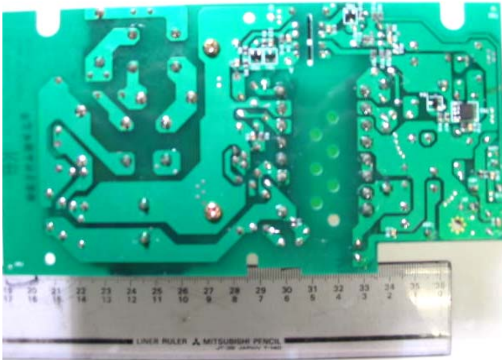
EUT PCB Trace Side
