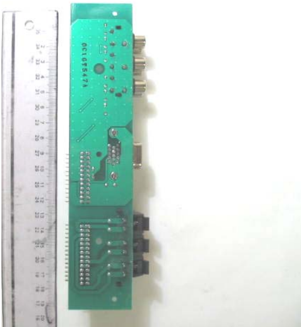
EUT PCB Trace Side
