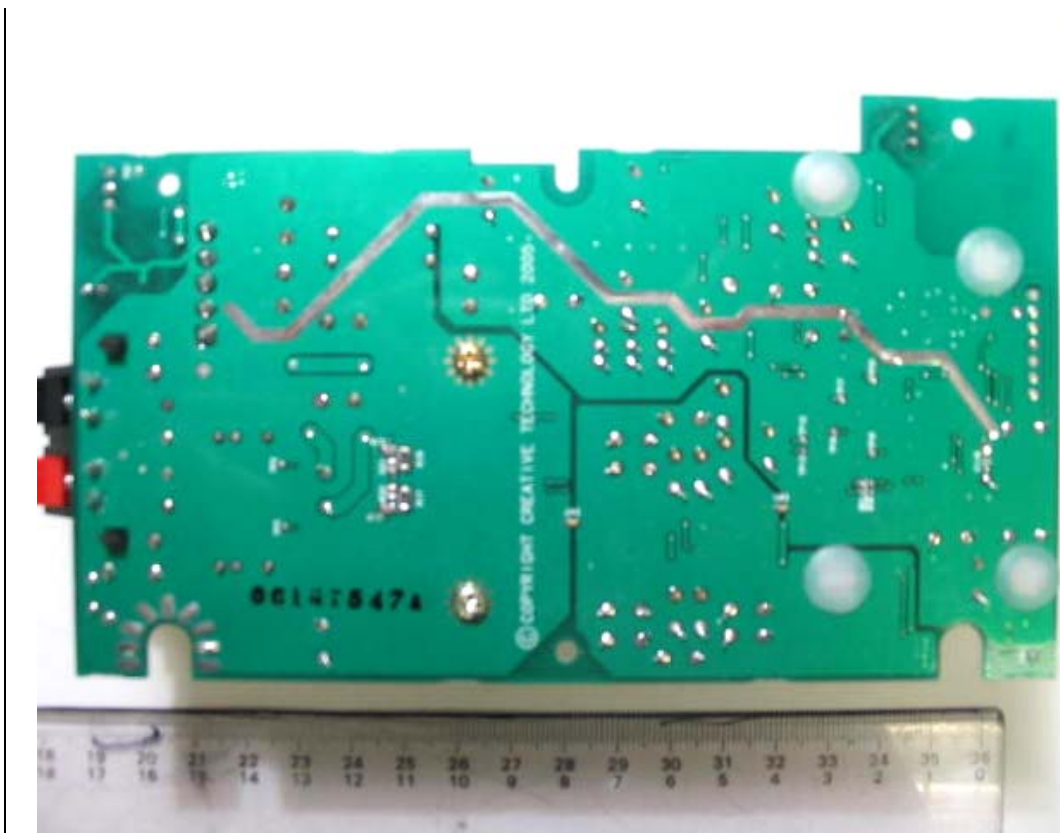
EUT PCB Trace Side
