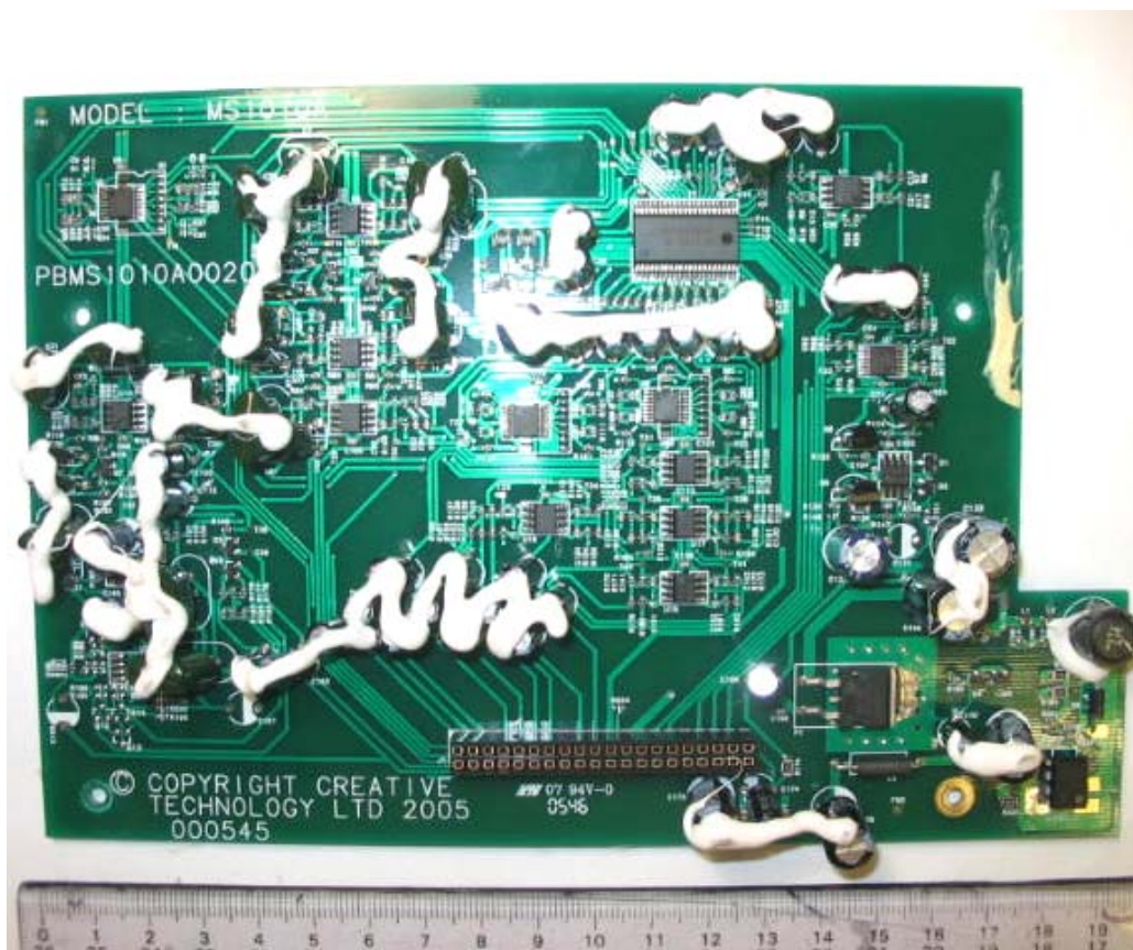
EUT PCB Component Side
