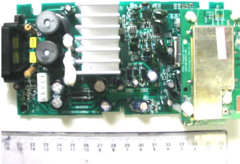
EUT PCB Component Side
