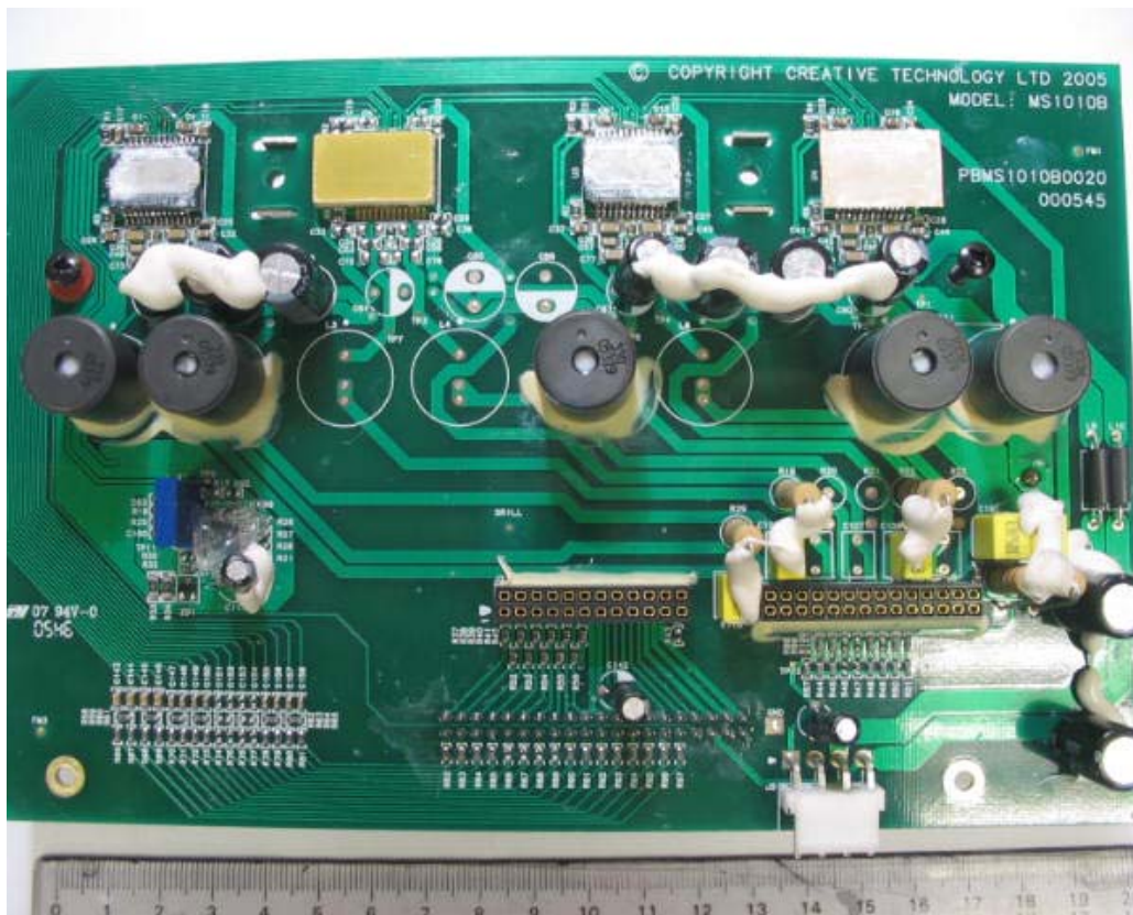
EUT PCB Component Side
