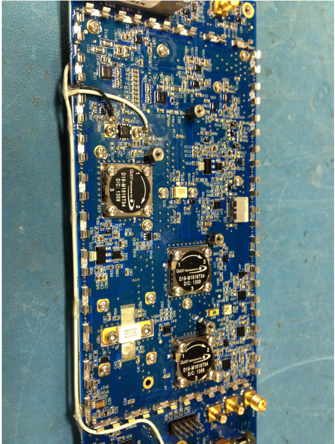
Figure 15: RFMM Board Top View (Circuitry Under the Metal Lid)
