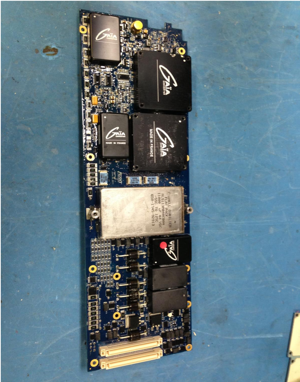
Figure 13: DAPM Board Bottom View
