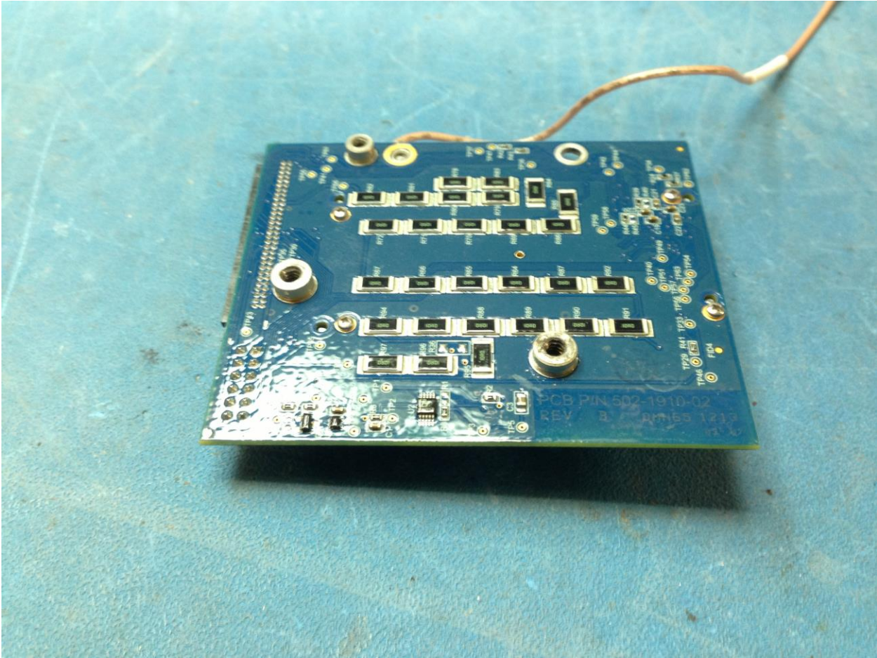
Figure 20: VMIM Board Bottom View
