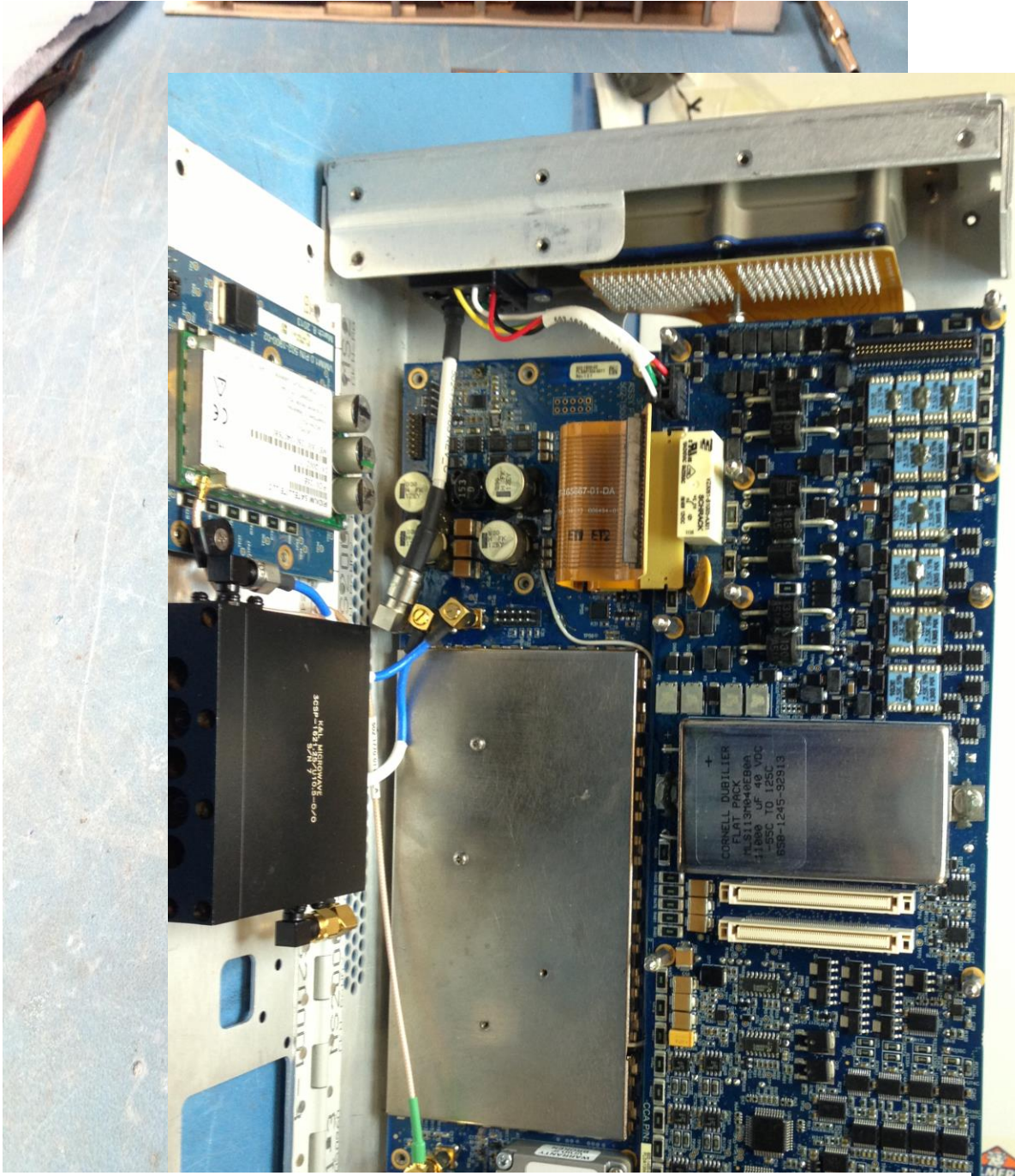
Figure 10: MCIM Top View Circuitry
