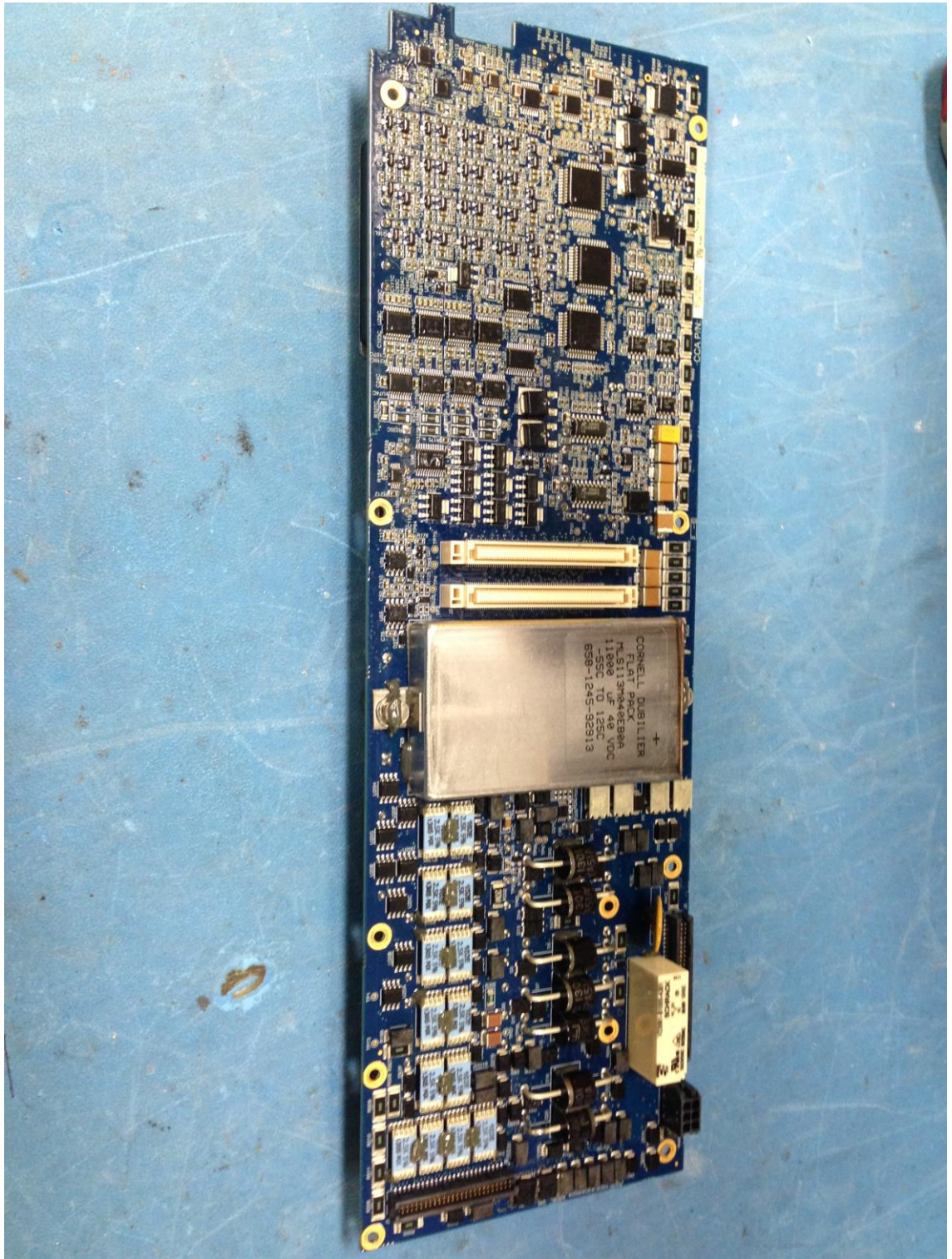
Figure 12: DAPM Board Top View
