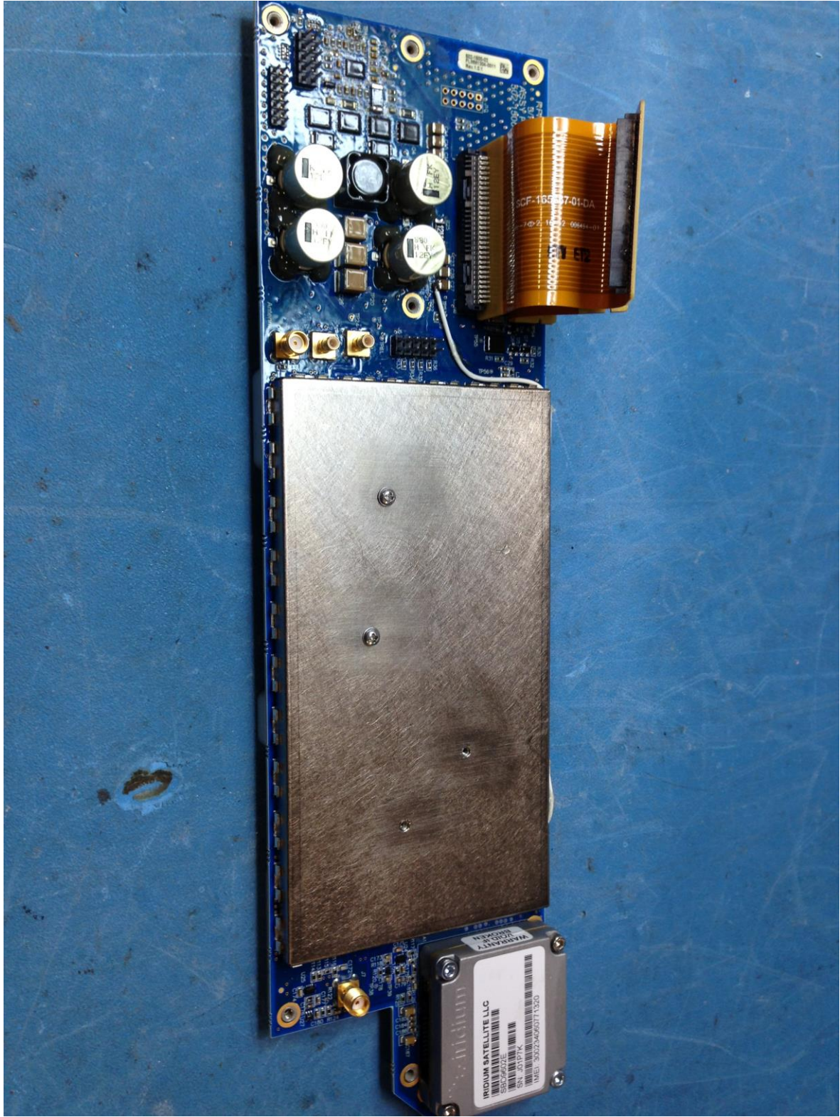
Figure 16: RFMM Board Top View
