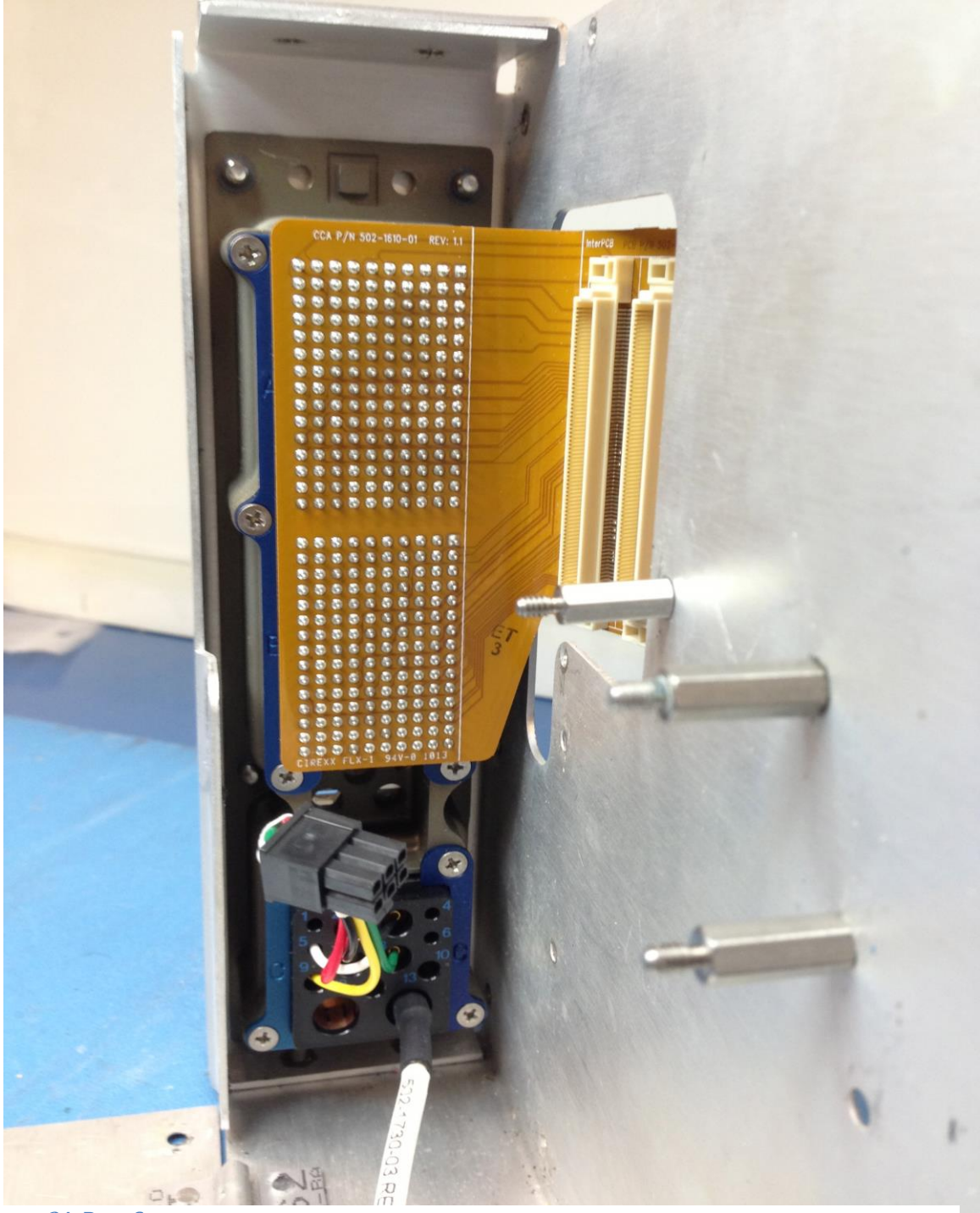
Figure 34: Rear Connector
