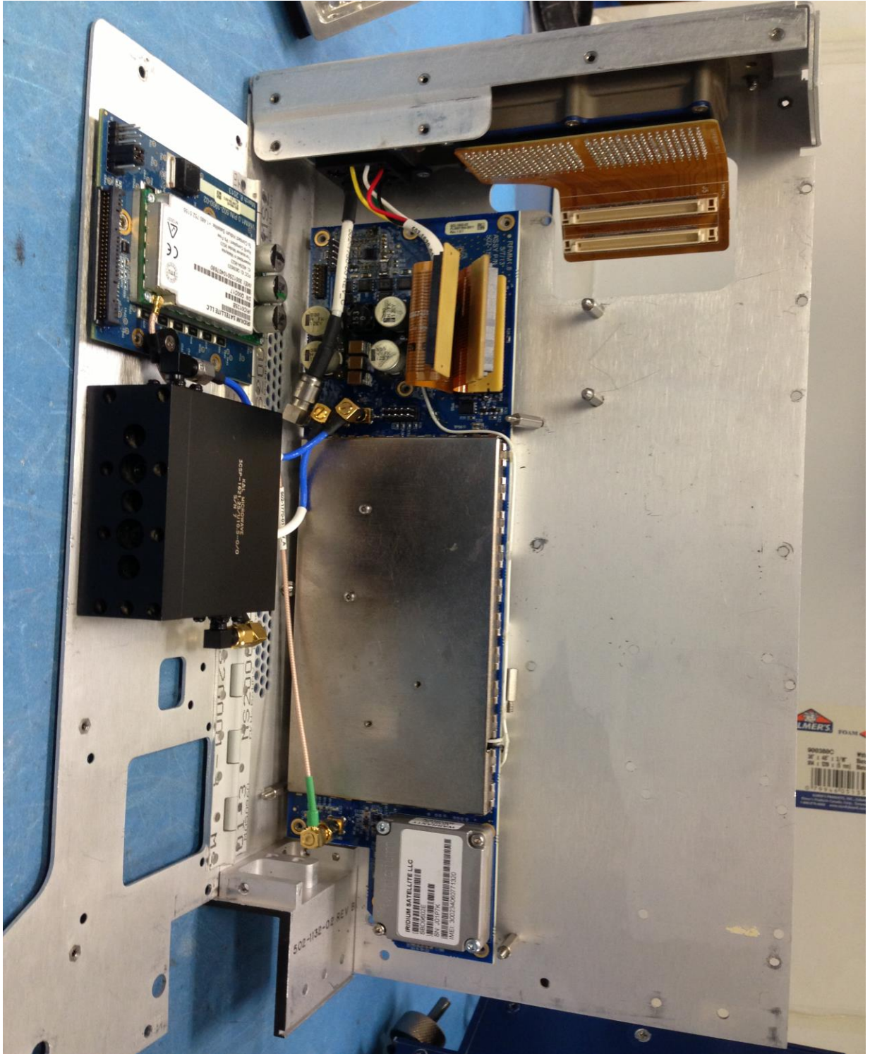
Figure 14: DAPM Board Removed
