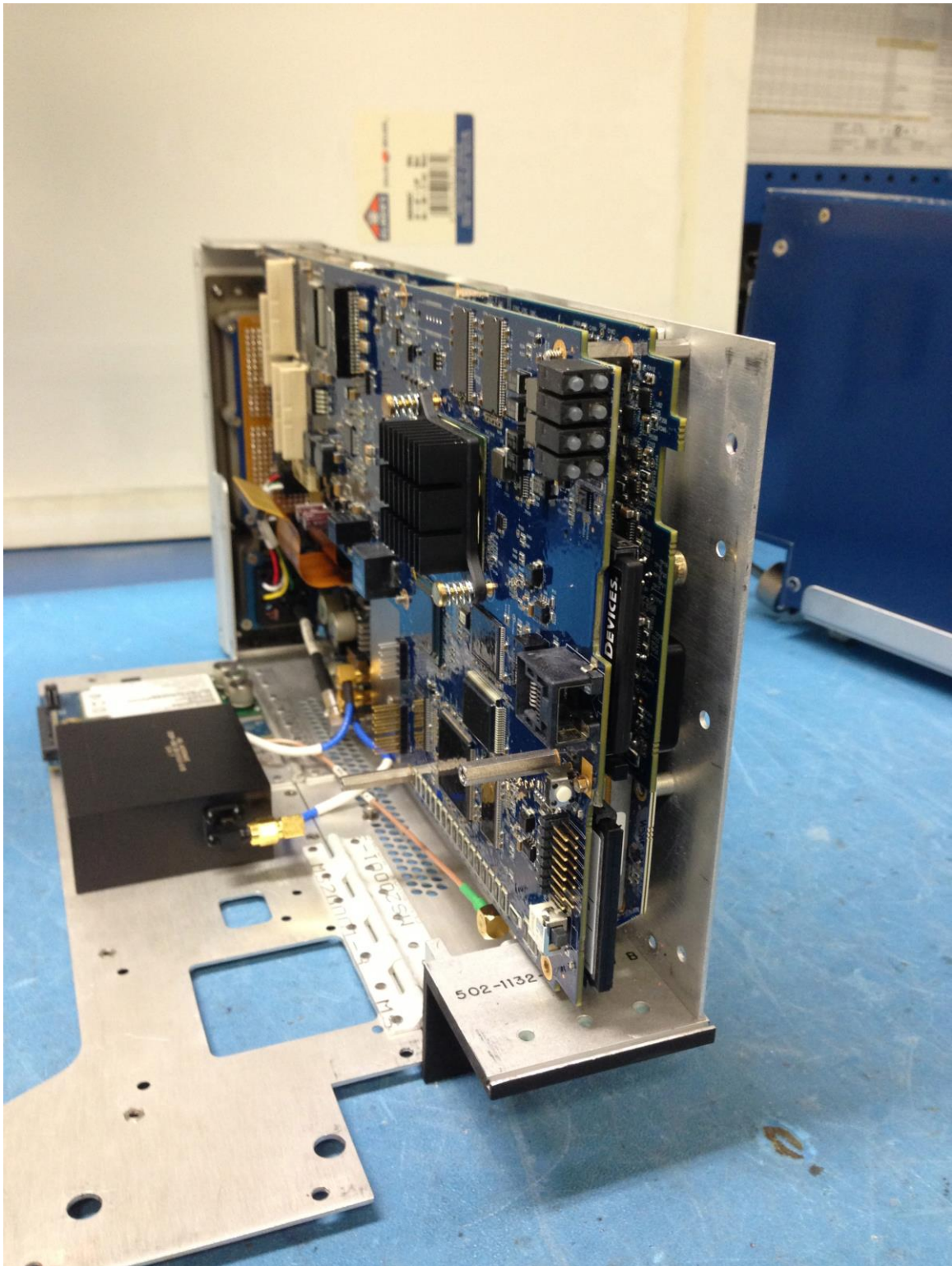
Figure 7: Front Panel Removed
