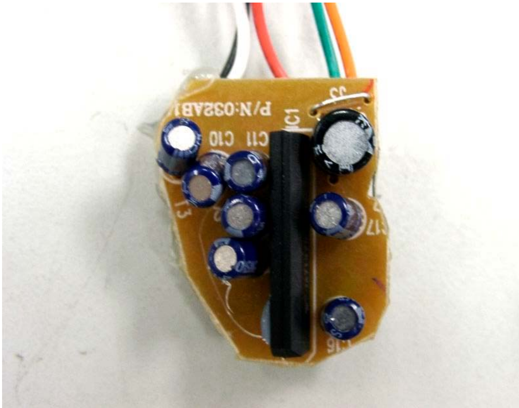
16. Front view of PCB 4
