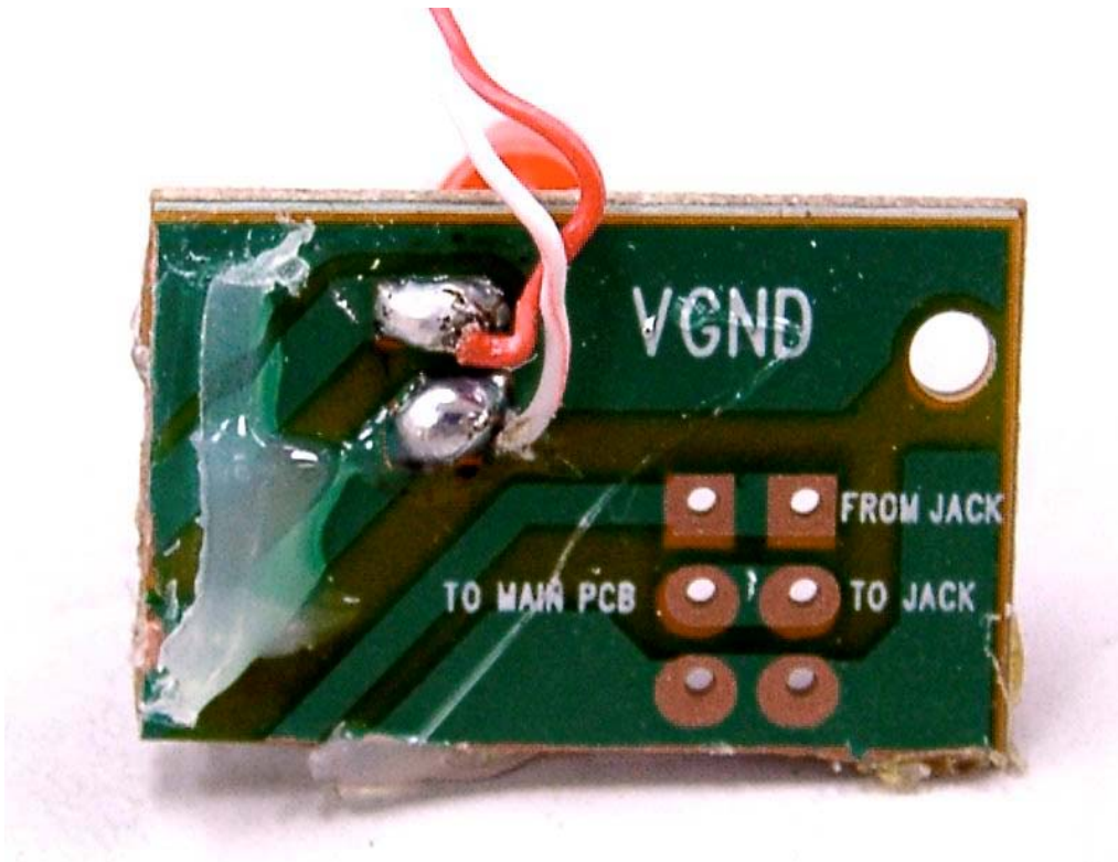
10. Rear view of PCB1
