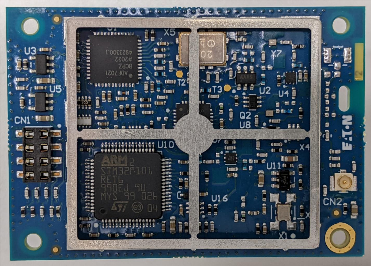
Figure 1 Top View of XPD900 (with RF Shield Lid Off)
