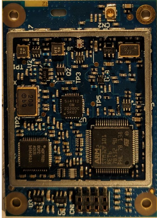
Figure 1 XPD900 board's top view with shield's lid removed.
