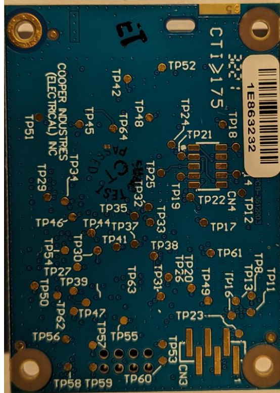
Figure 2 XPD900 back view
