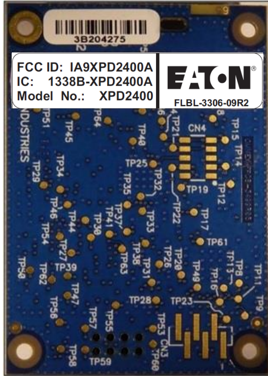
Figure 2 XPD2400 Back Picture with FCC & IC Label
