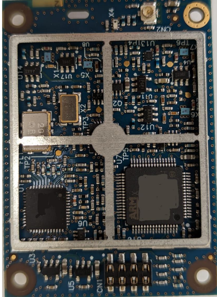
Figure 1 XPD2400 board's top view with shield's lid removed.
