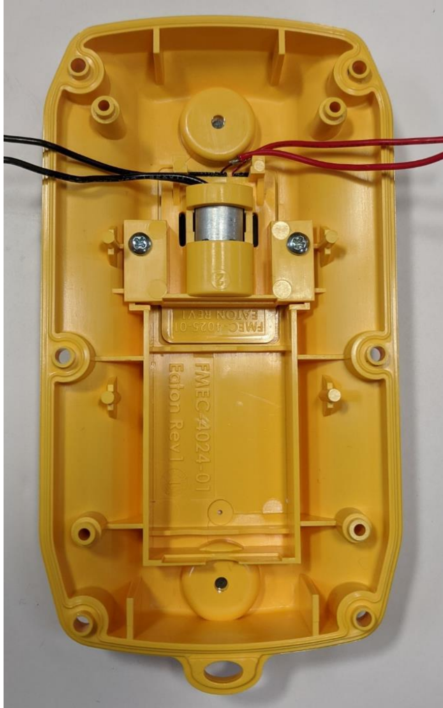
Figure 4 TD110-2.4 GHz Back Shell Assembly.
