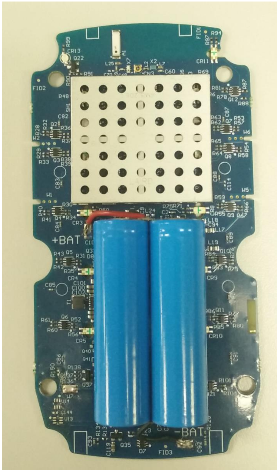
Figure 2 TD110-2.4 GHz PCB bottom with battery and RF shield installed.
