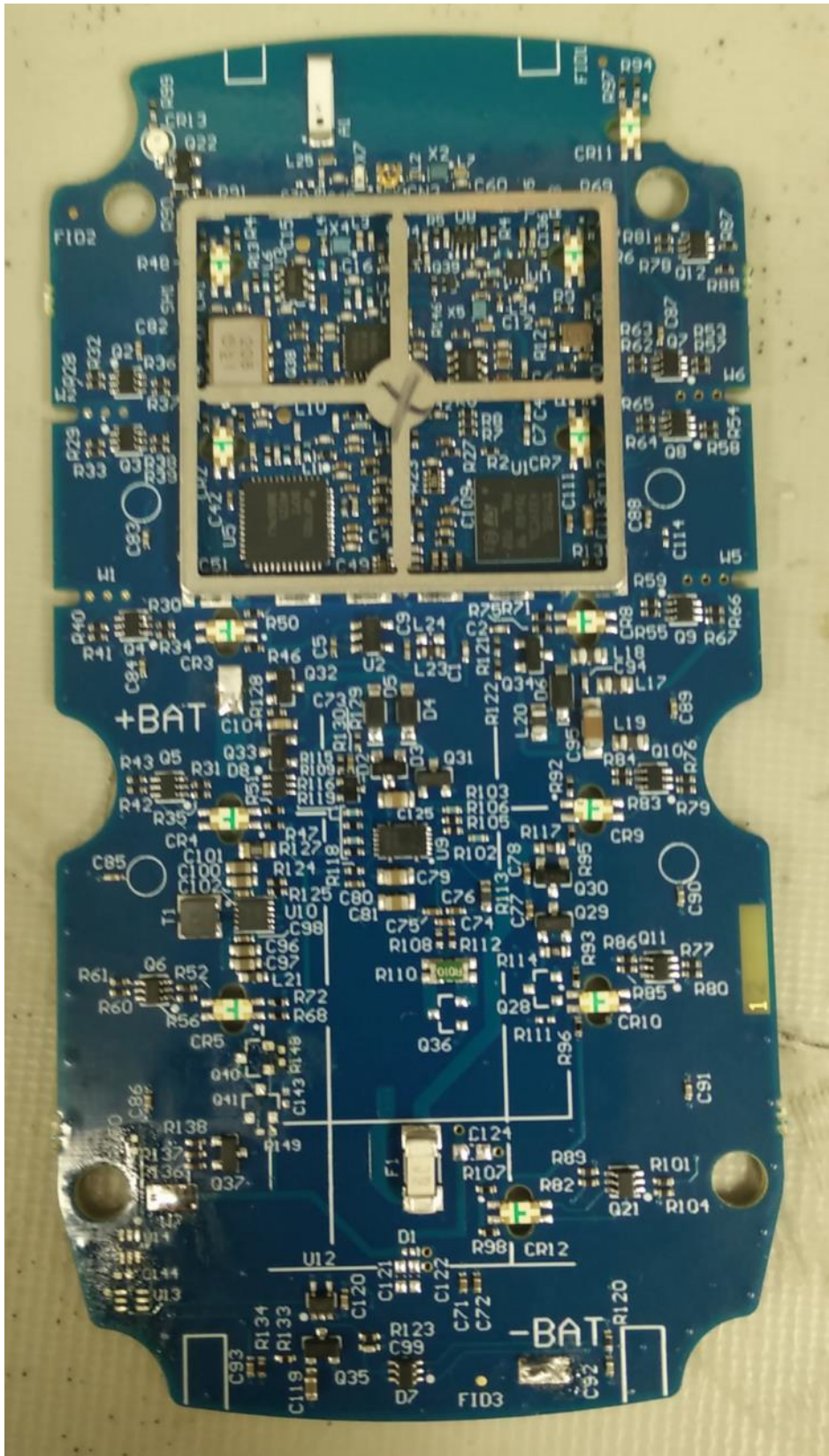
Figure 3 TD110-2.4 GHz PCB bottom view.
