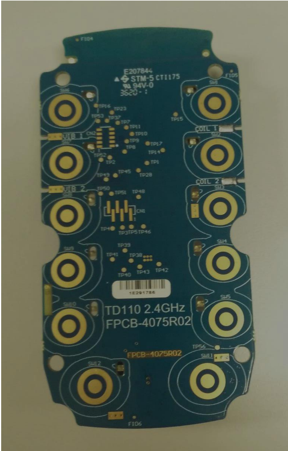
Figure 1 TD110-2.4 GHz PCB top view with key domes removed.
