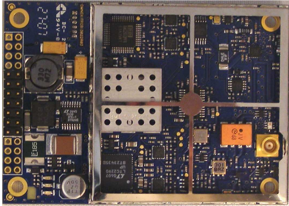
6.3 MR-900 Transceiver Module Top Side, Main Shield Removed:
