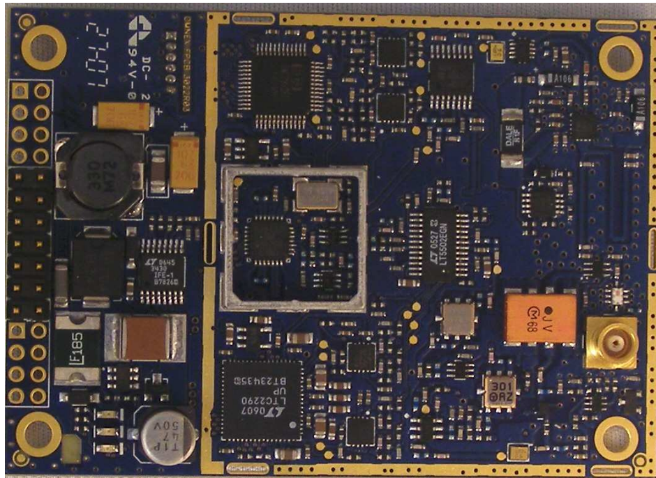
6.4 MR-900 Transceiver Module Top Side, All Shields Removed:
