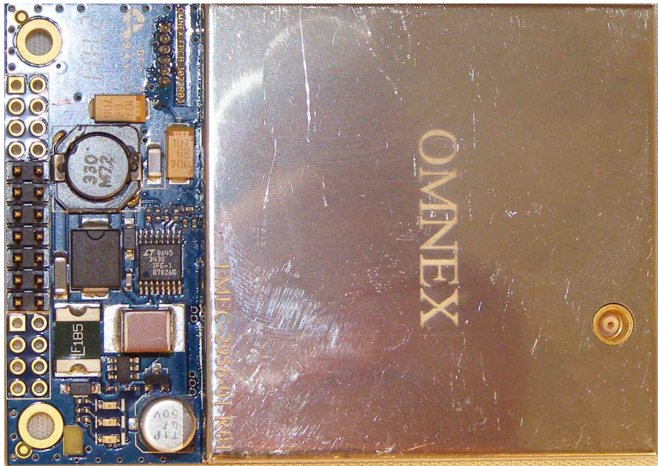
6.1 MR-900 Transceiver Module Top Side with Shield Installed:
