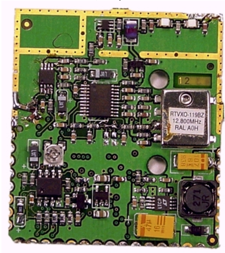
Module; Component side
