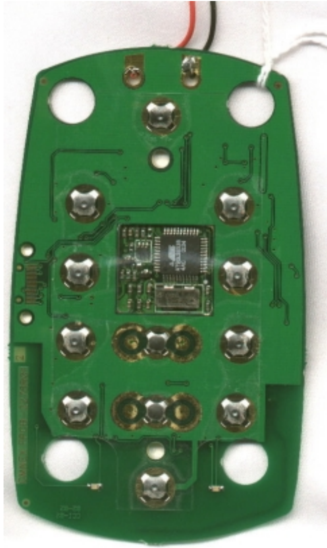
Module installed on Processor board: Foil Side
