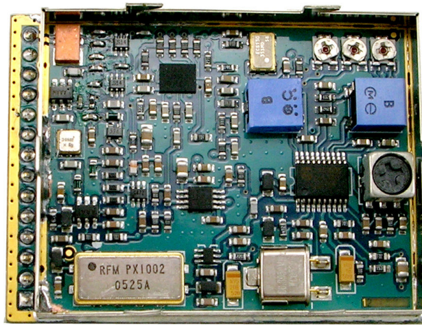
LPD-24RC Transceiver Module Top Side Shield Removed:
