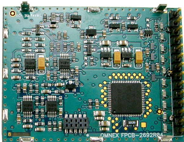
LPD-24RC Transceiver Module Bottom Side:
