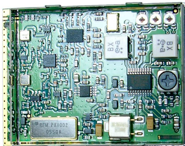
6.2 HPD-24RC Transceiver Module Top Side Shield Removed:
