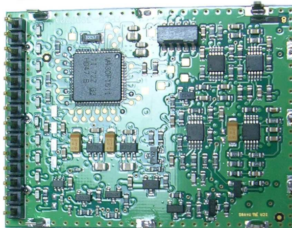
6.3 HPD-24RC Transceiver Module Bottom Side:
