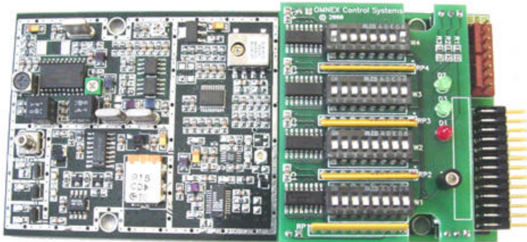
DEX-900 Transceiver All shields removed
