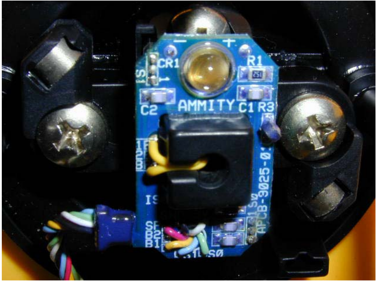
APCB-9025-01 BOARD 2
