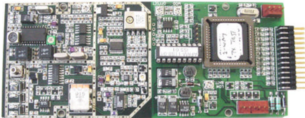
T245 Transceiver All shields removed
