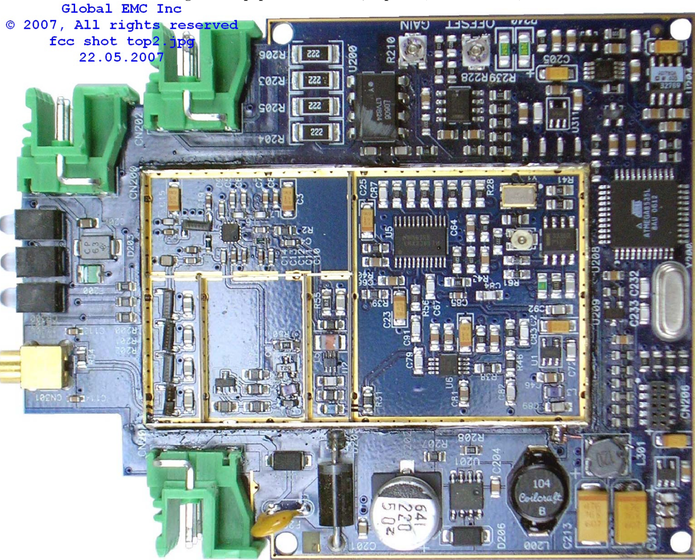
Figure 3 - Equipment Under Test, Top Side (Shield Removed)
