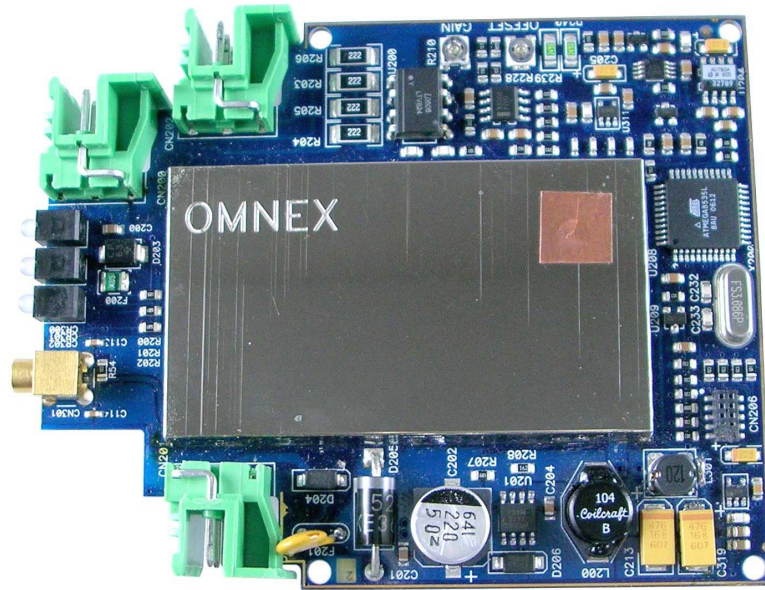
Top Internal View
