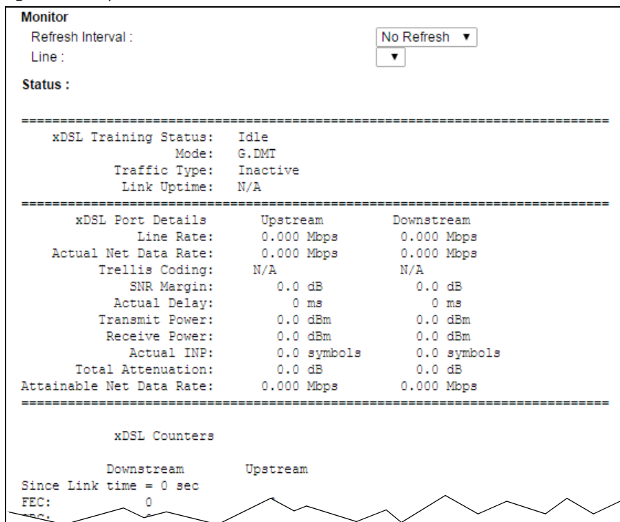
Figure 137 System Monitor > xDSL Statistics
