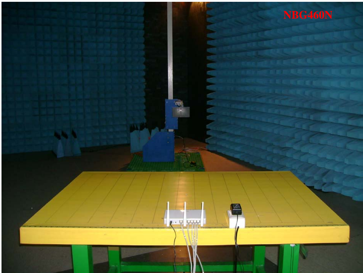
Photo 4: Radiated Emission Test set-up photo
