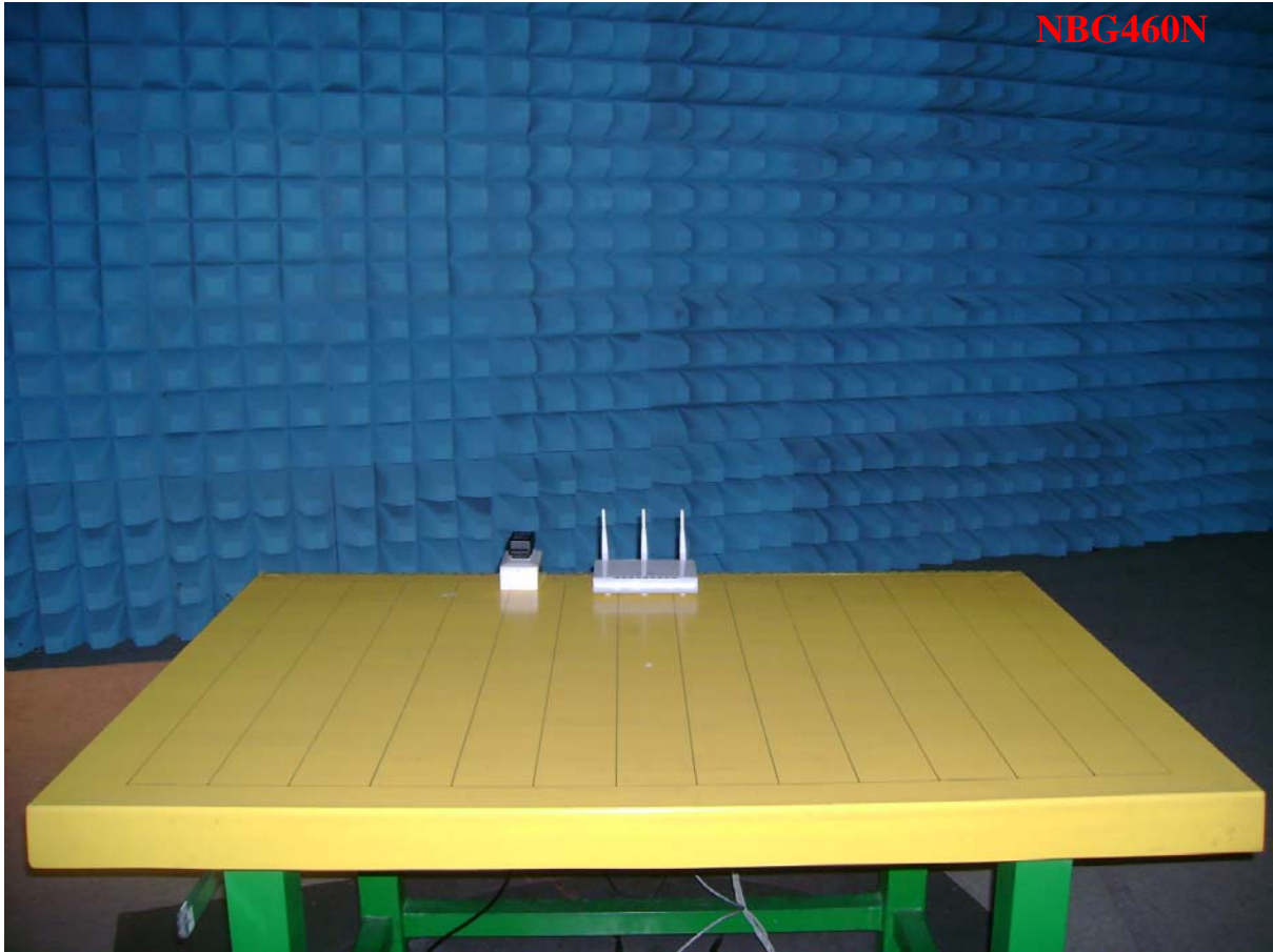
Photo 3: Radiated Emission Test set-up photo
