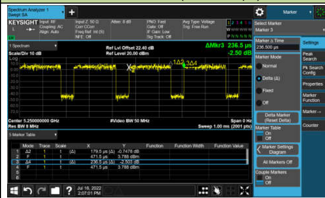
802.11ax-HE160 (T = 179.5µs)
