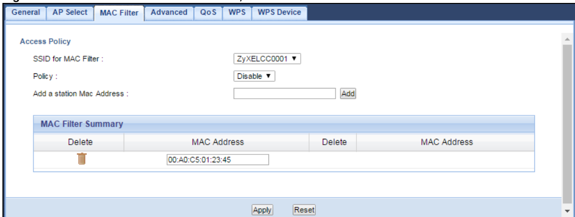
Figure 35 Network > Wireless LAN 2.4G/5G > MAC Filter
