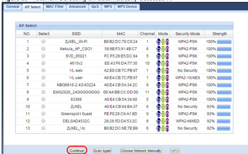
Figure 20 Tutorial: Selecting an automatically detected AP
