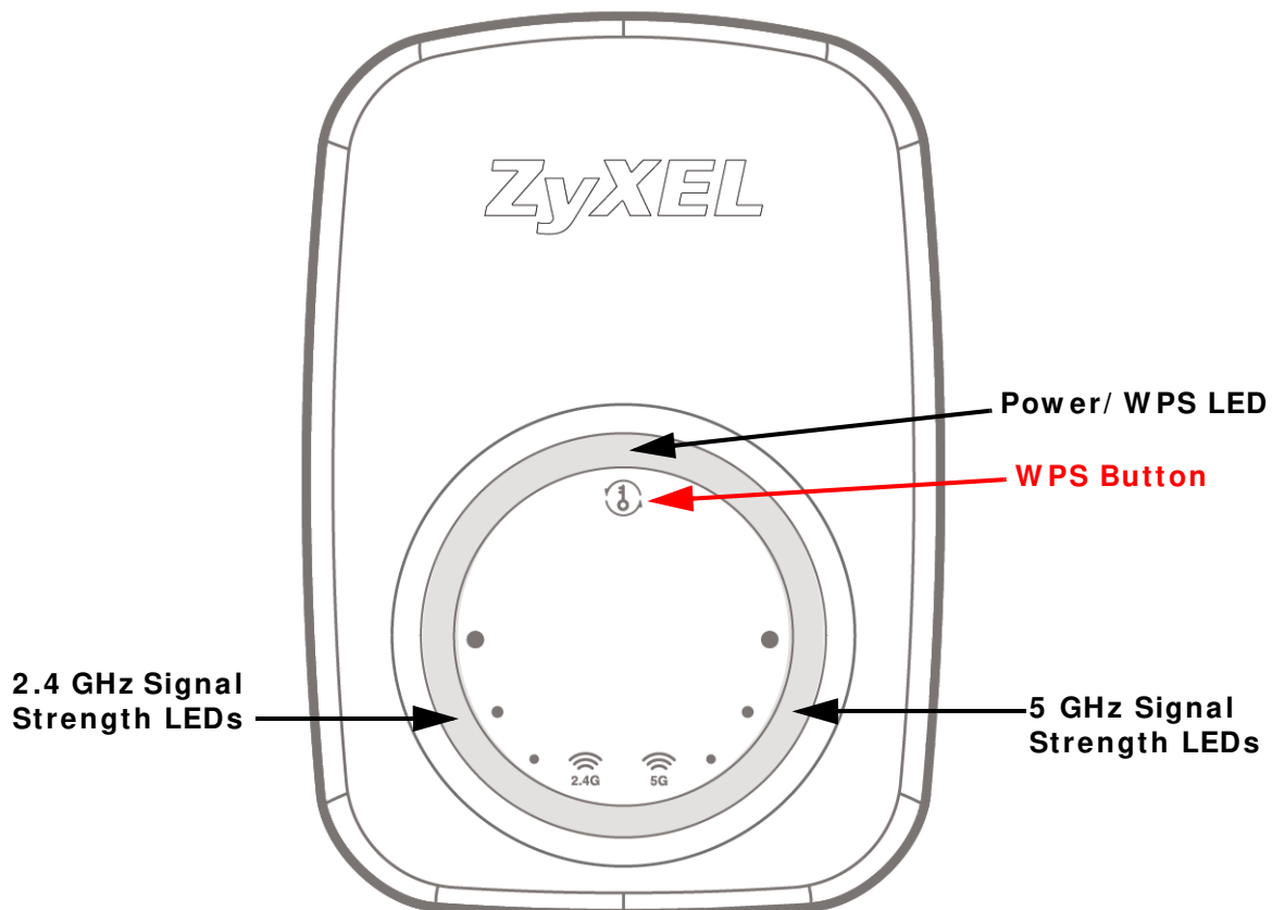
Figure 2 Front Panel
