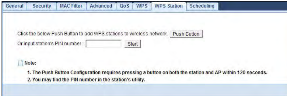
Figure 47 Network > Wireless LAN (2.4/5G) > WPS Station
