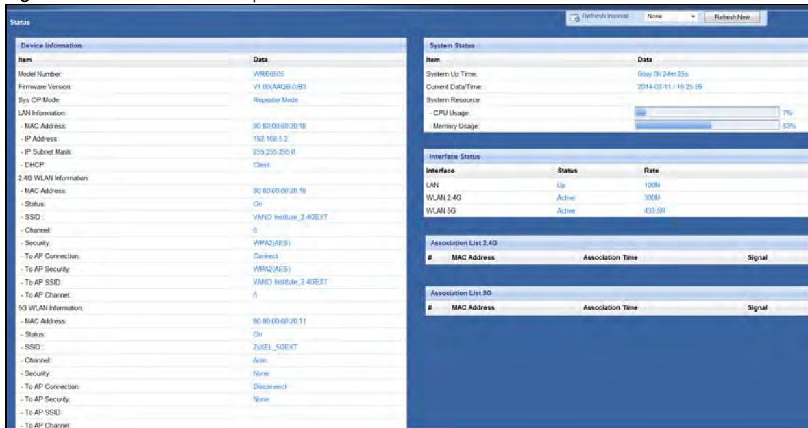
Figure 7 Status: Universal Repeater Mode
