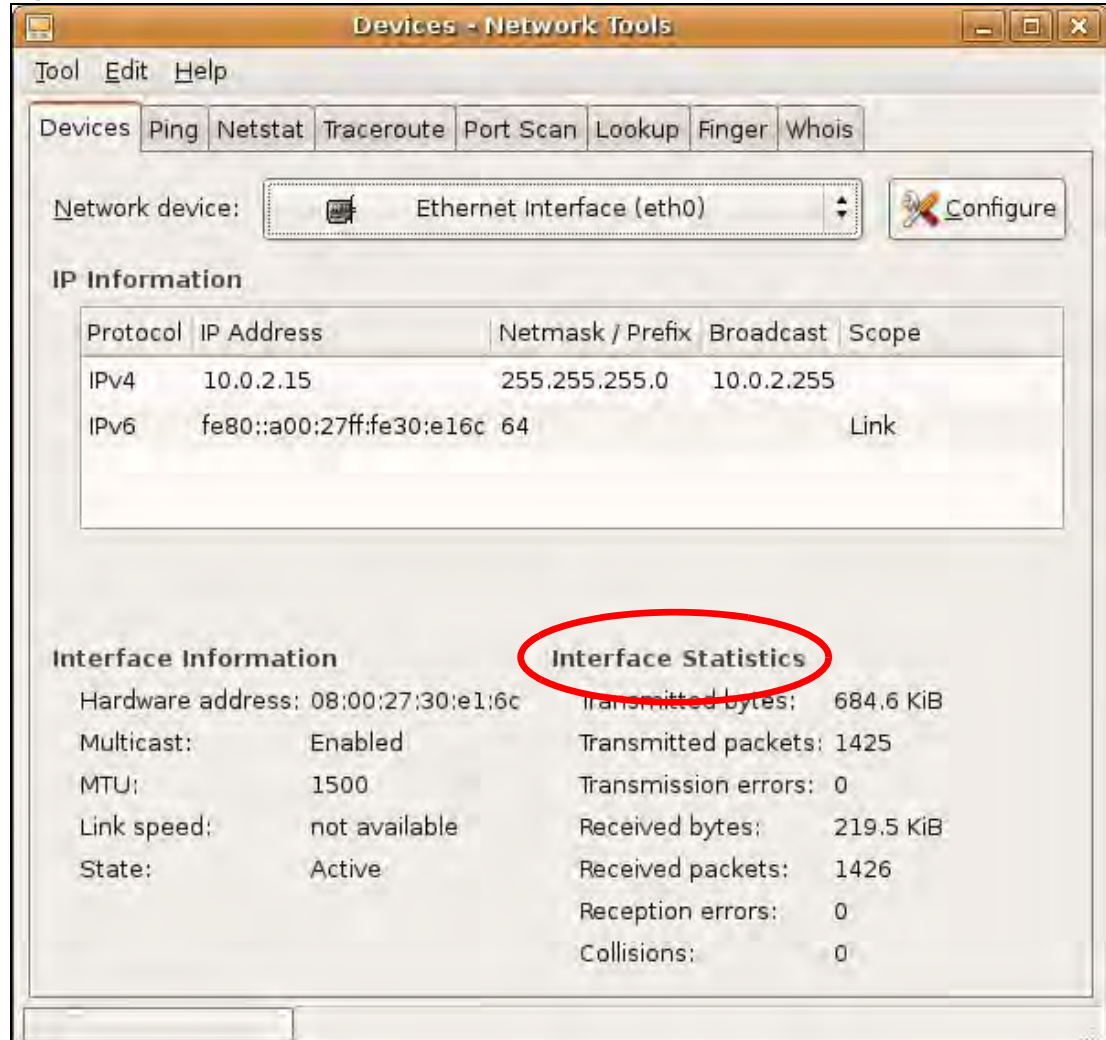
Figure 66 Ubuntu 8: Network Tools
