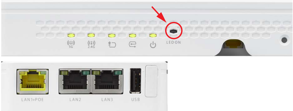
Figure 8 WAC5302D-S LEDs
