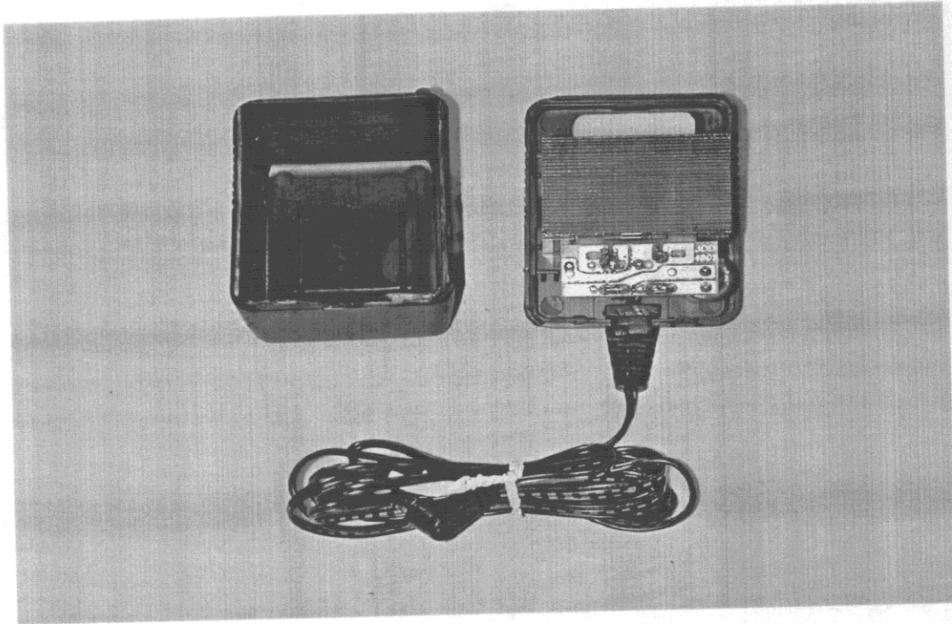
Inner View of Adapter
