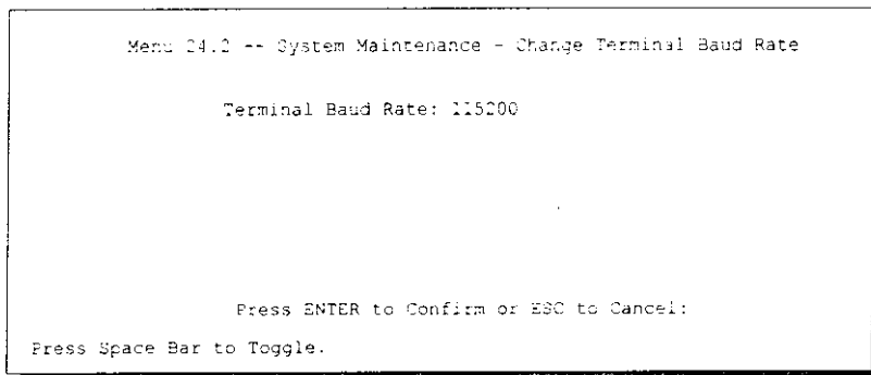
Figure 10-4. Menu 24.2 - System Maintenance - Change Terminal Baud Rate
