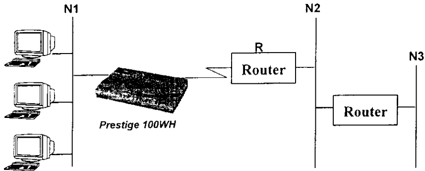
Figure 5-4. Example of Static Routing Topology
