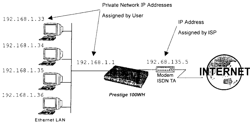
Figure 3-5. Single User Account Topology
