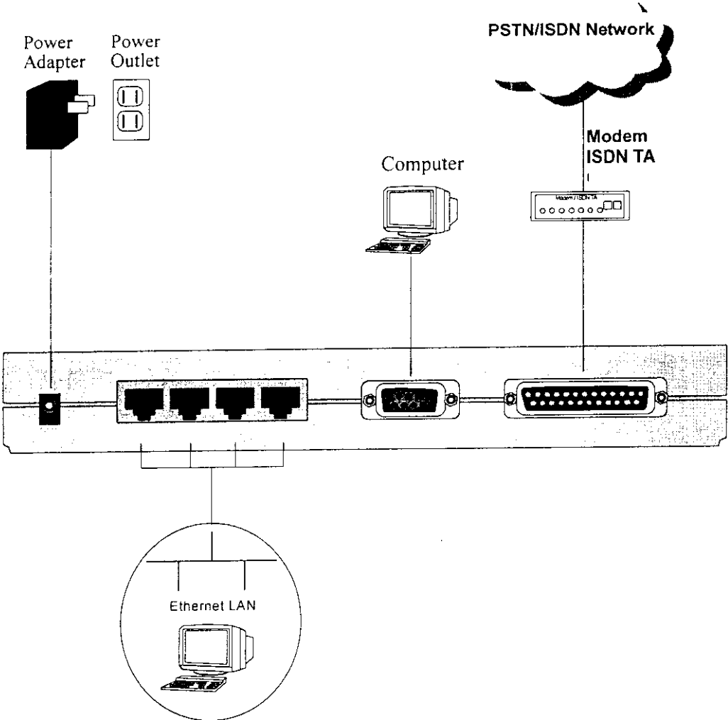
Figure 2-1. Connect Prestige 100WH
