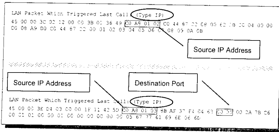
Figure 10-3. LAN Packet Which Triggered Last Call
