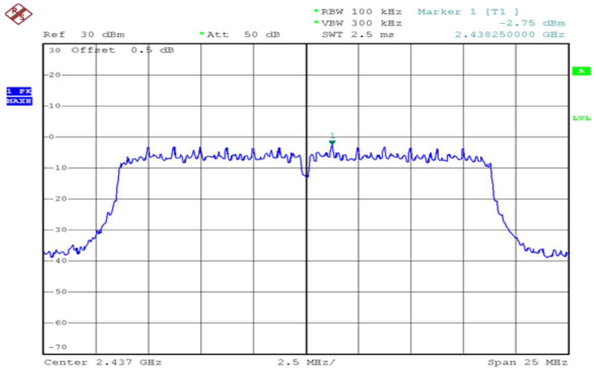
Channel 06 (2437MHz)
