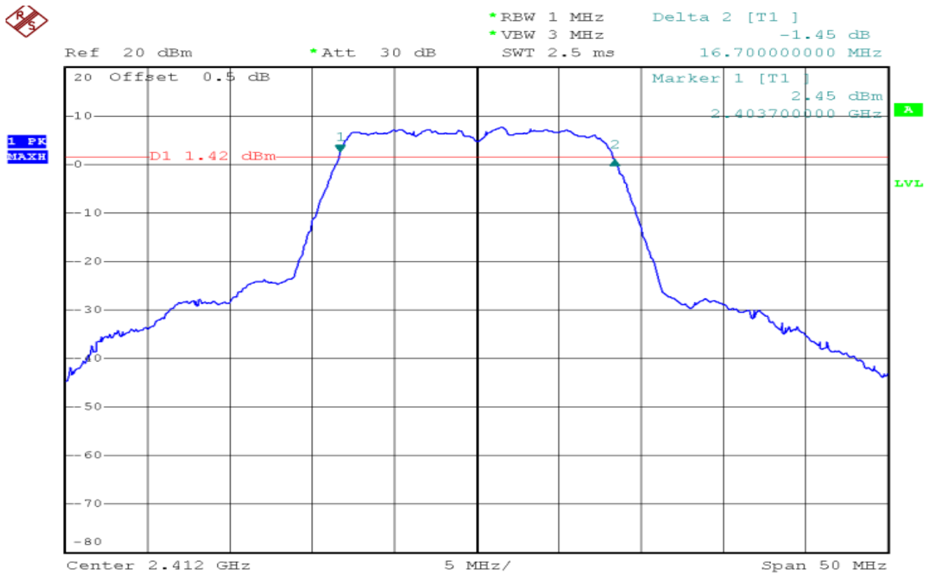
Channel 01 (2412MHz)
