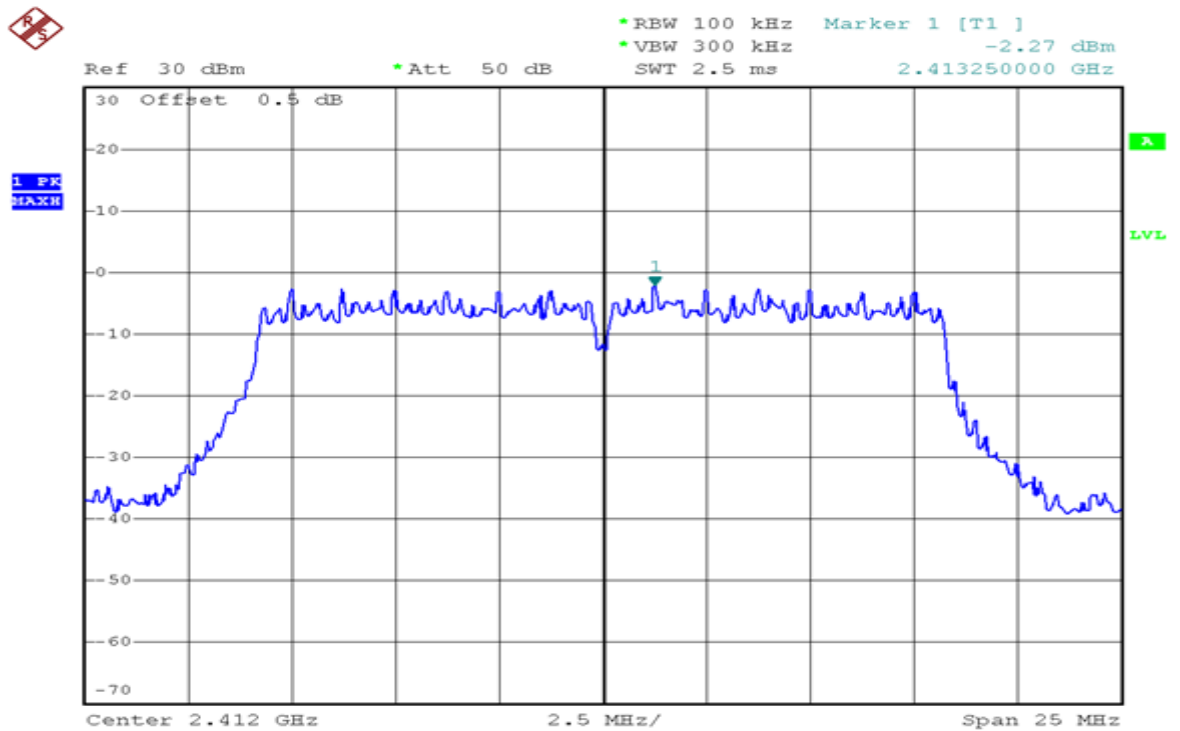
Channel 01 (2412MHz)
