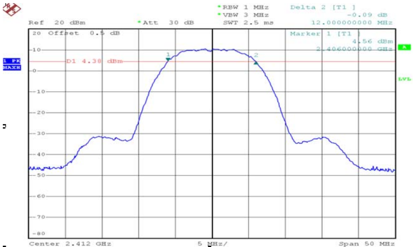
Channel 01 (2412MHz)
