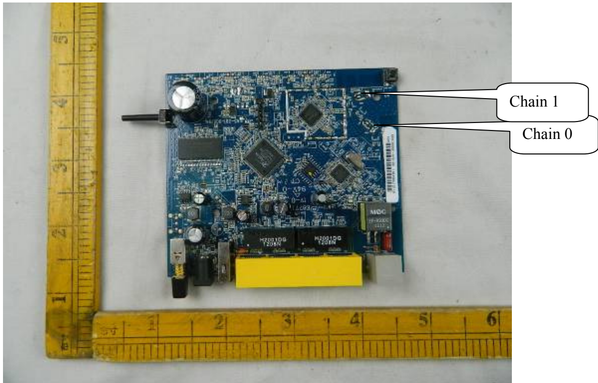
4) EUT Photo(with PCB antenna)
