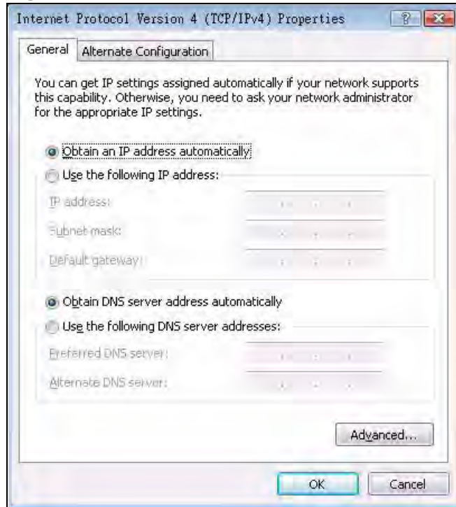
Figure 133 Windows Vista: Internet Protocol Version 4 (TCP/IPv4) Properties
