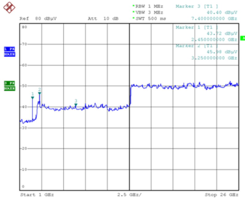
Channel 03 (2422MHz)
