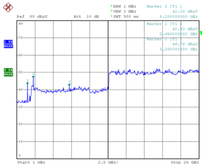
Channel 06 (2437MHz)
