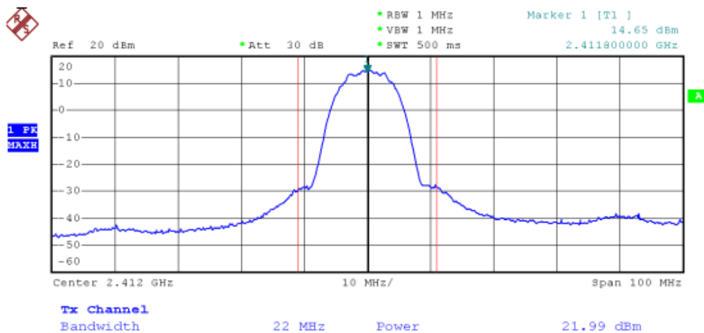
Channel 01 (2412MHz)
