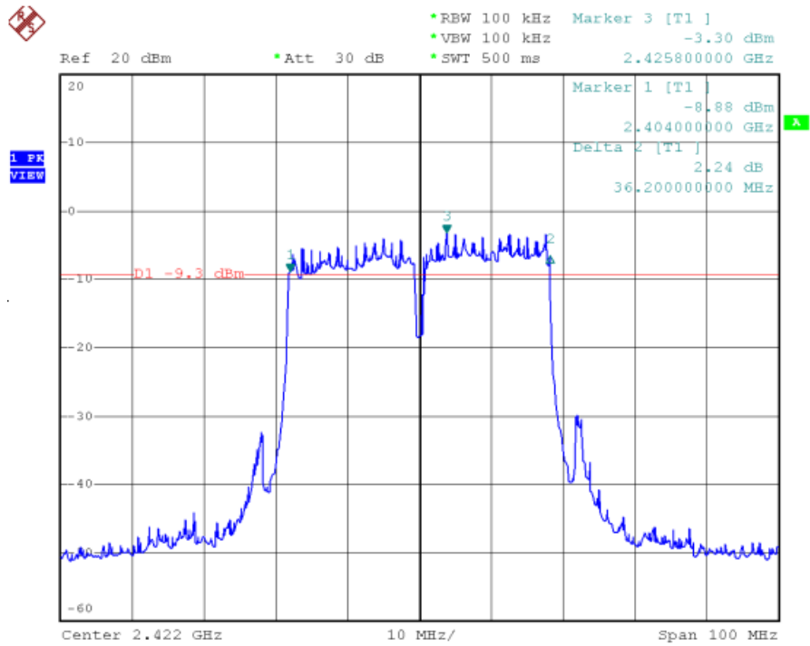
Channel 03 (2422MHz)
