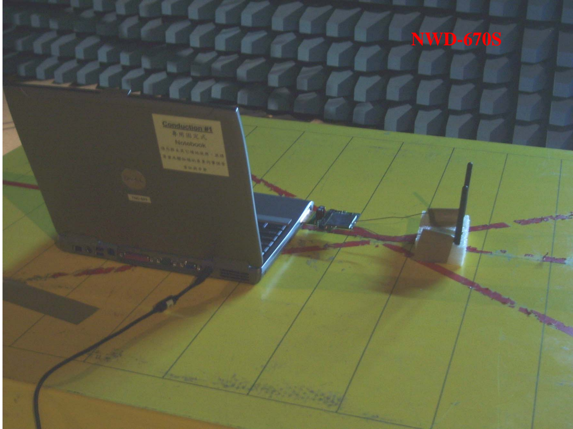
Photo 2: Radiated Emission Test Set-up
