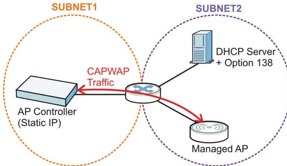
Figure 24 CAPWAP and DHCP Option 138
