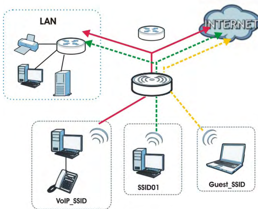
Figure 2 Multiple BSSs
