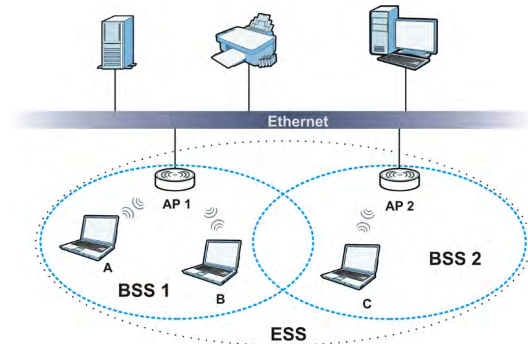
Figure 93 Infrastructure WLAN
