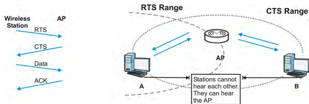
Figure 94 RTS/CTS
