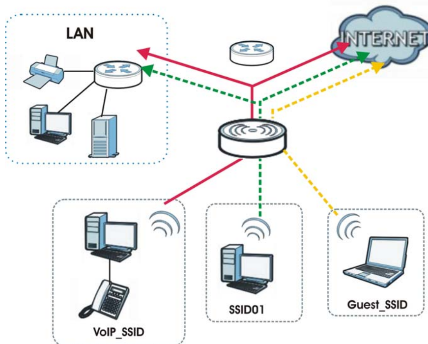
Figure 1 Multiple BSSs
