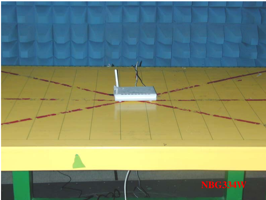
Photo 1: Radiated Emission Test set-up photo
