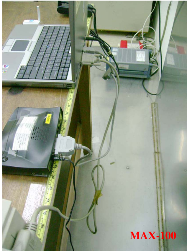
Photo 2: Conducted Emission Test Set-up photo
