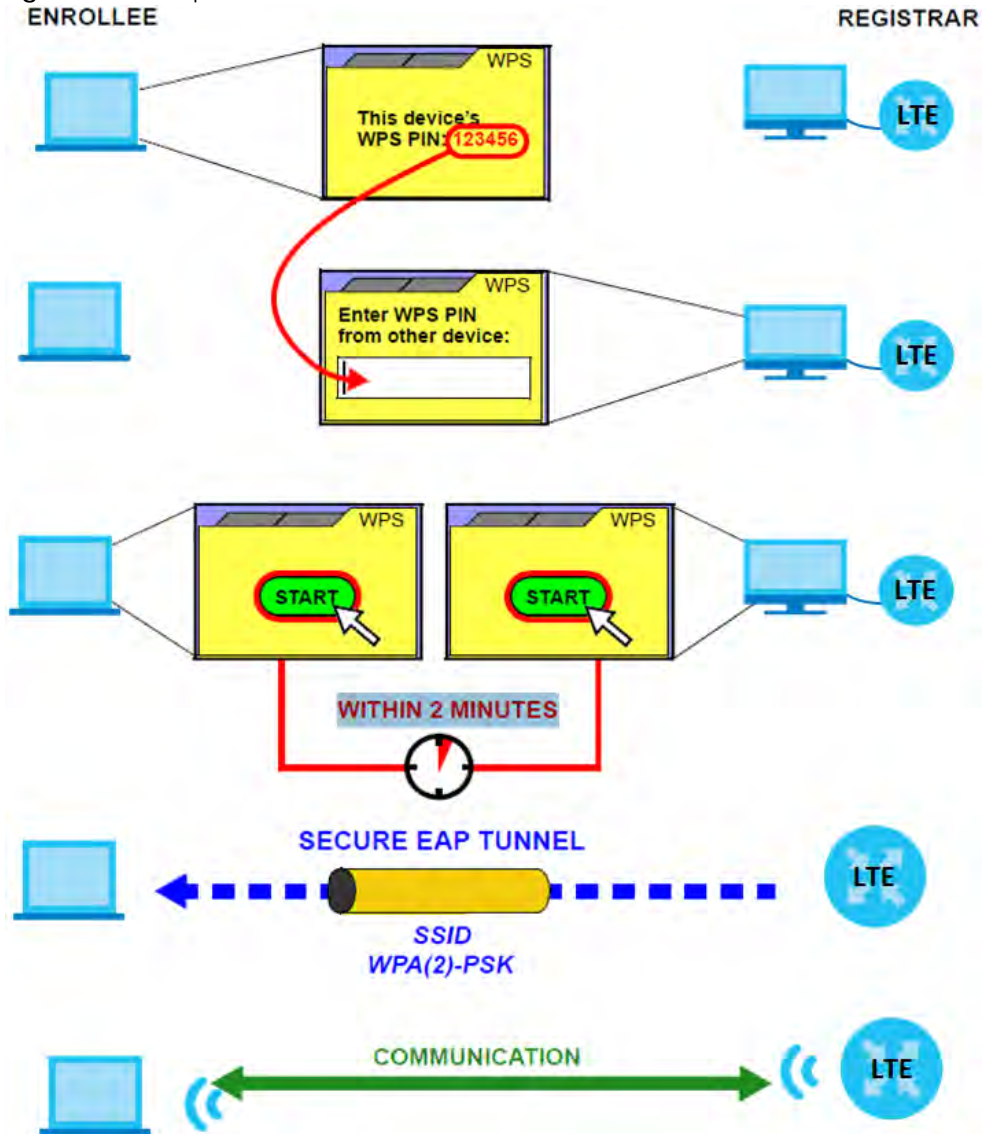
Figure 90 Example WPS Process: PIN Method ENROLLEE
