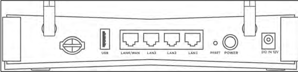
Figure 12 Bottom Panel (LTE7240-M403)
