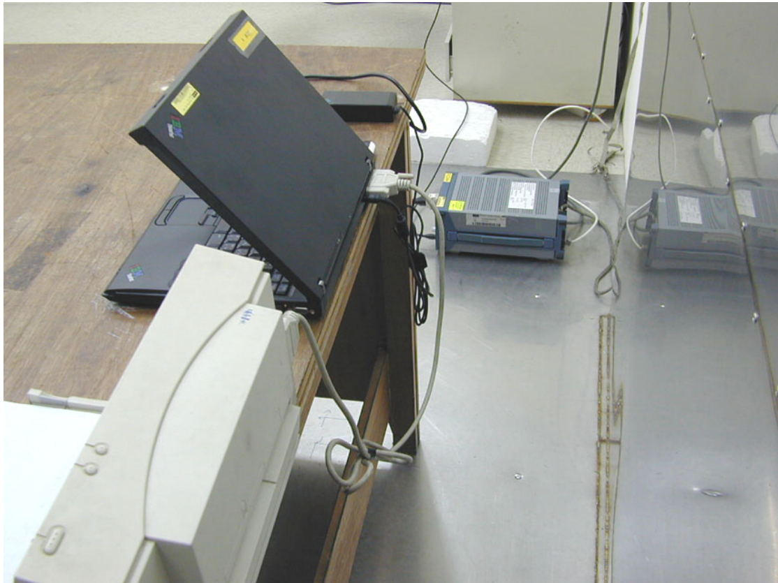
Photo 3: Conducted Emission Test Set-up photo
