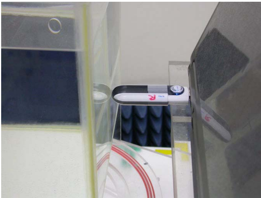
Figure 11: EUT perpendicular to phantom, 0 mm separation- Zoom In
