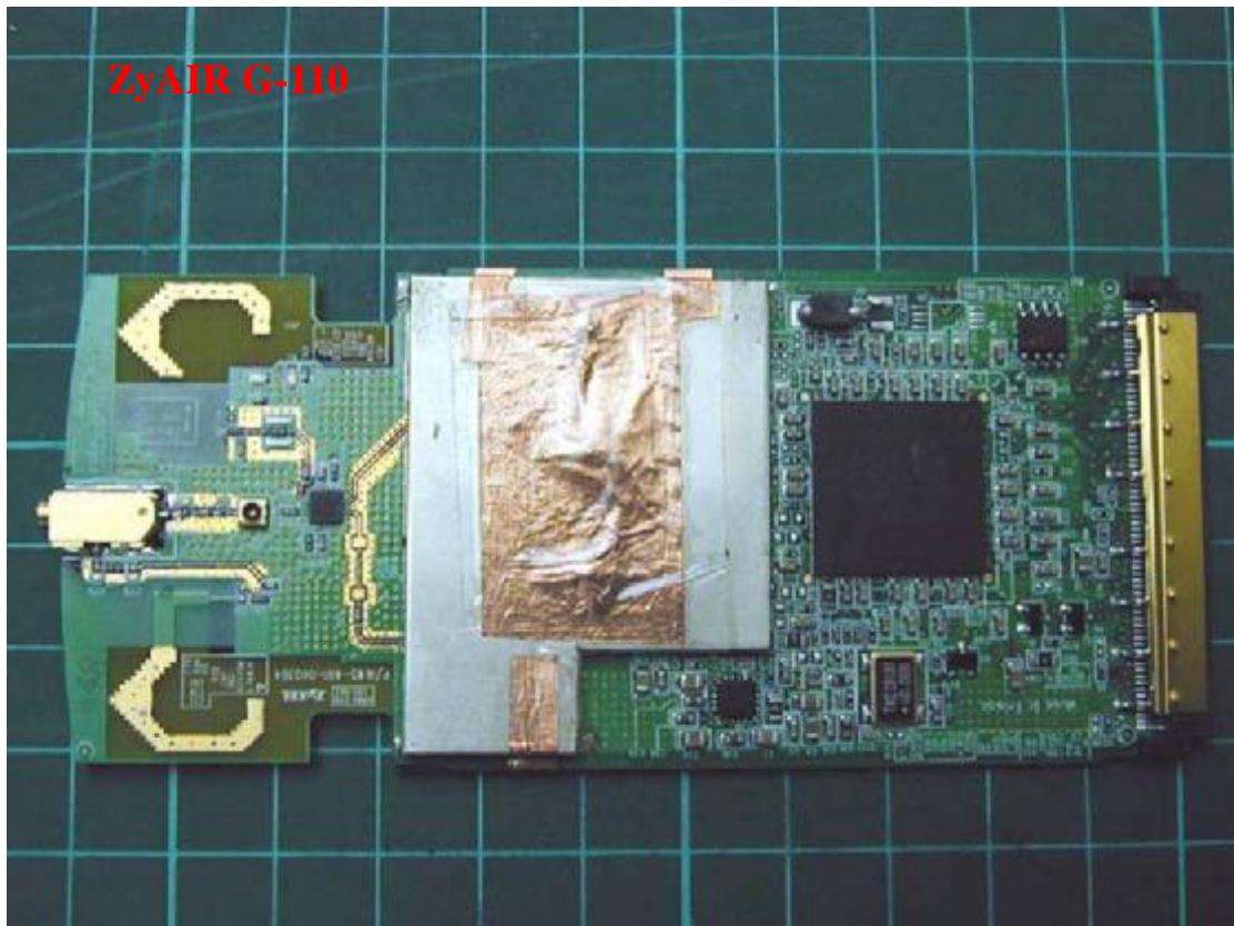
Photo 1: Internal photo
