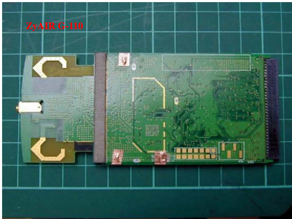
Photo 4: Internal photo
