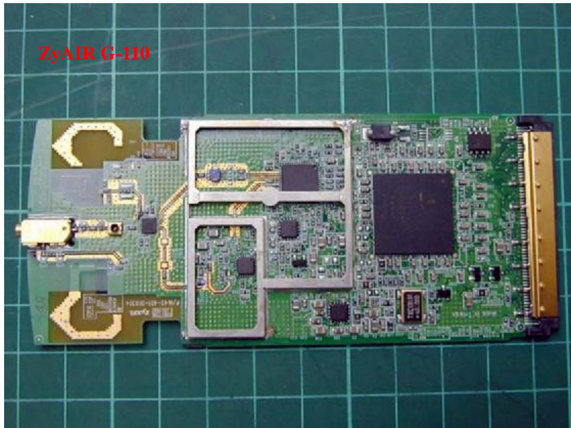
Photo 2: Internal photo
