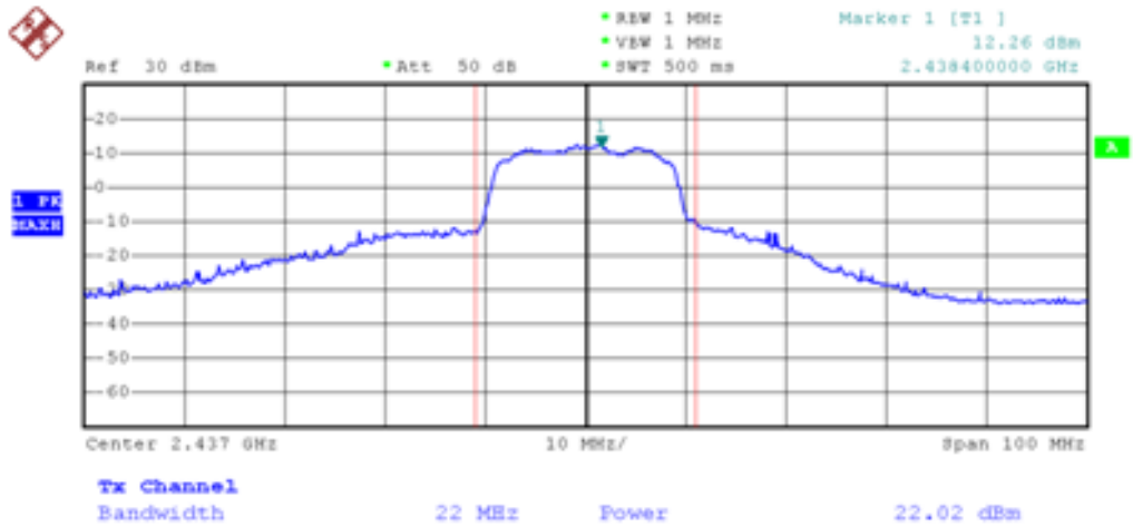
Channel 06 (2437MHz) (An1)
