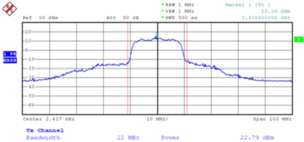
Channel 06 (2437MHz) (An0)
