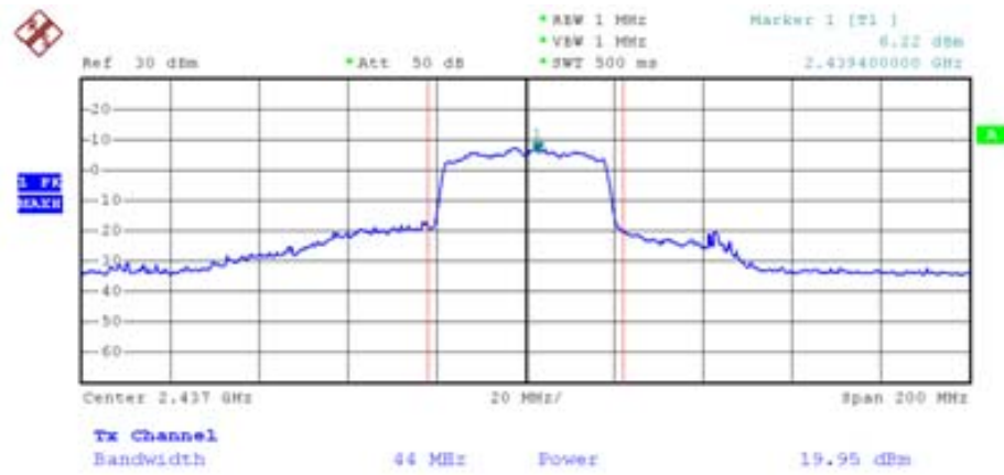
Channel 06 (2437MHz) (An0)
