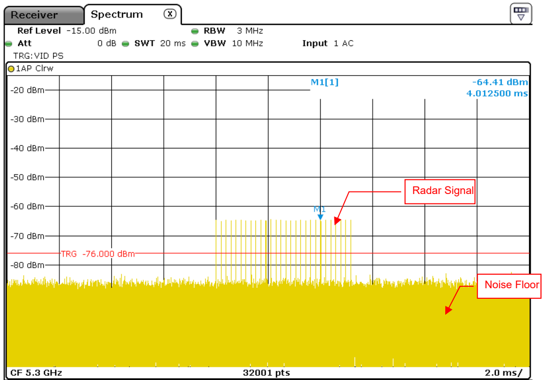
Radar Signal 2
