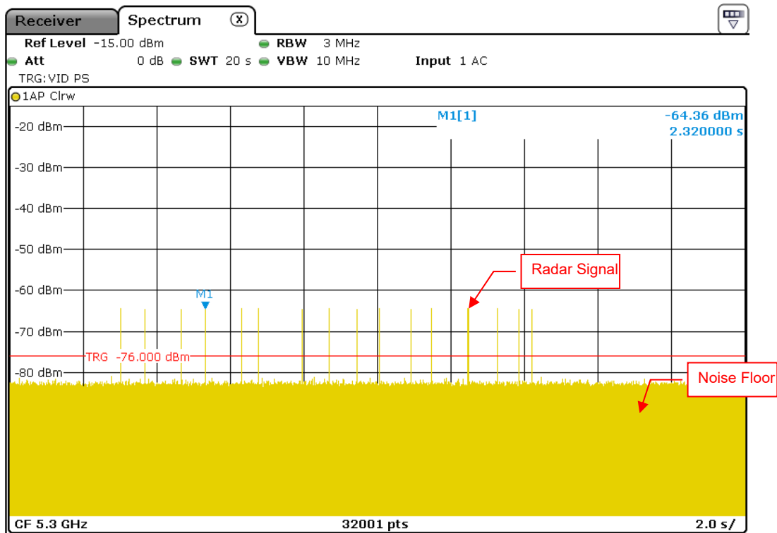
Radar Signal 5
