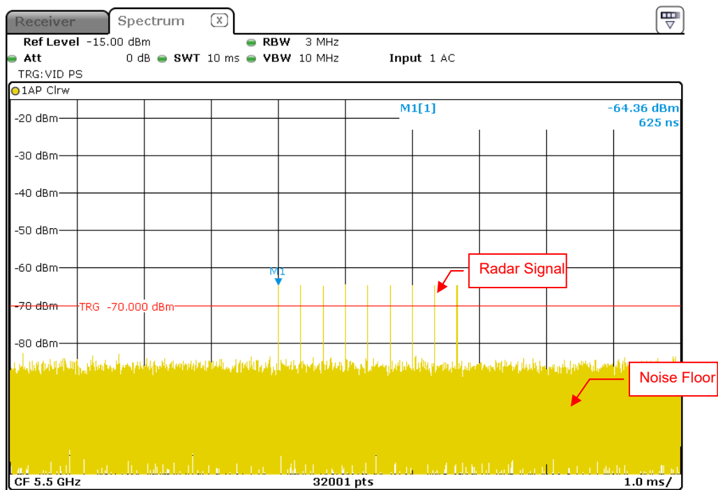
Radar Signal 6
