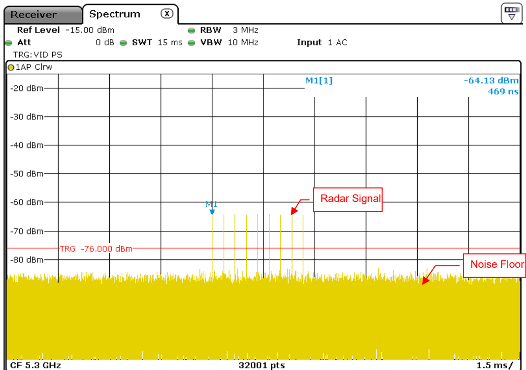
Radar Signal 6
