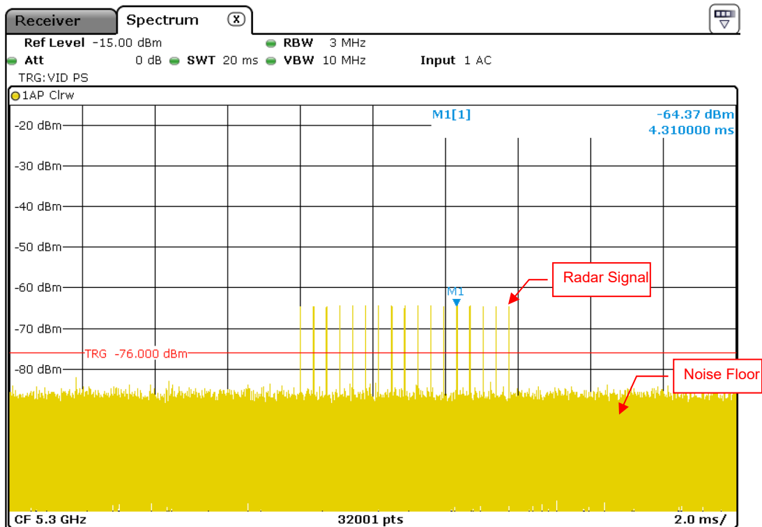
Radar Signal 3
