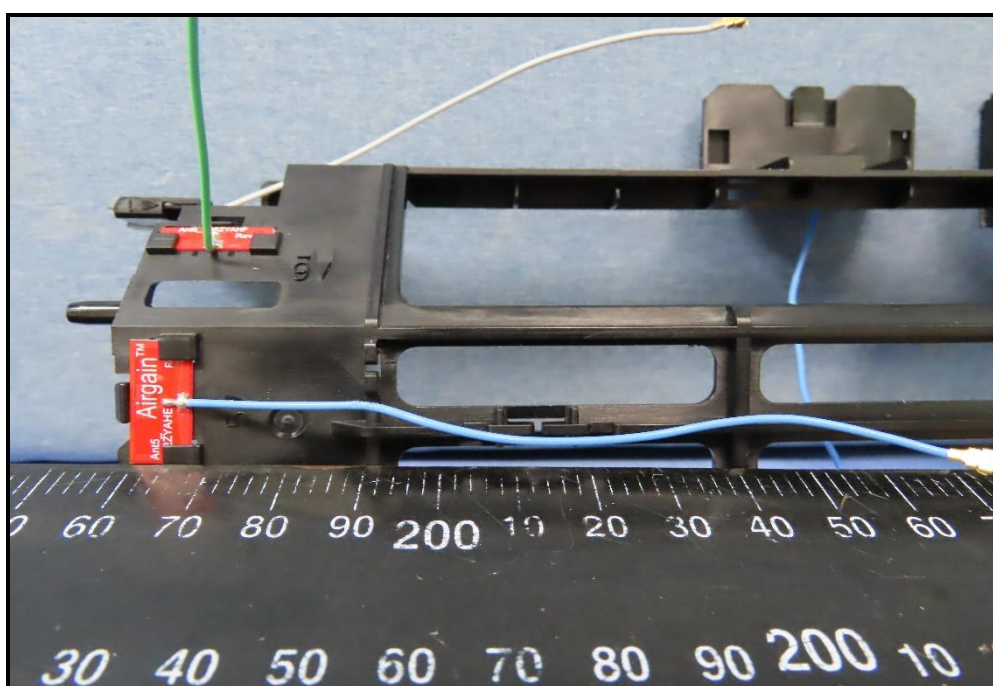
Antenna NO.5
