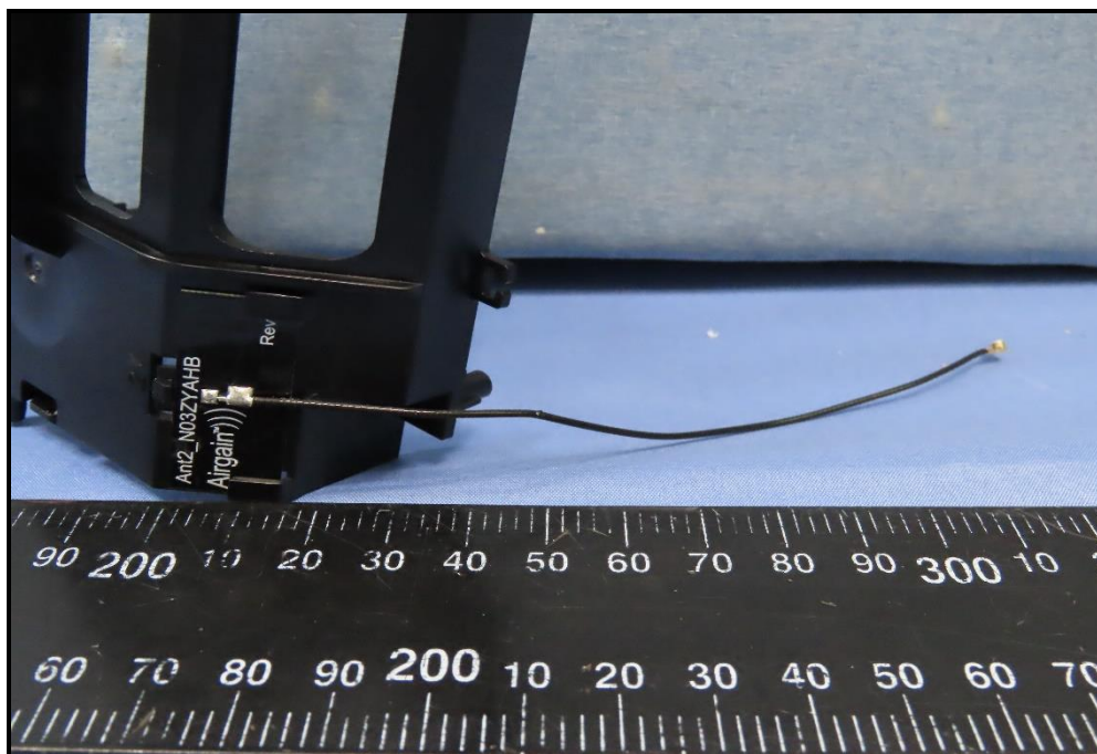
Antenna NO.2
