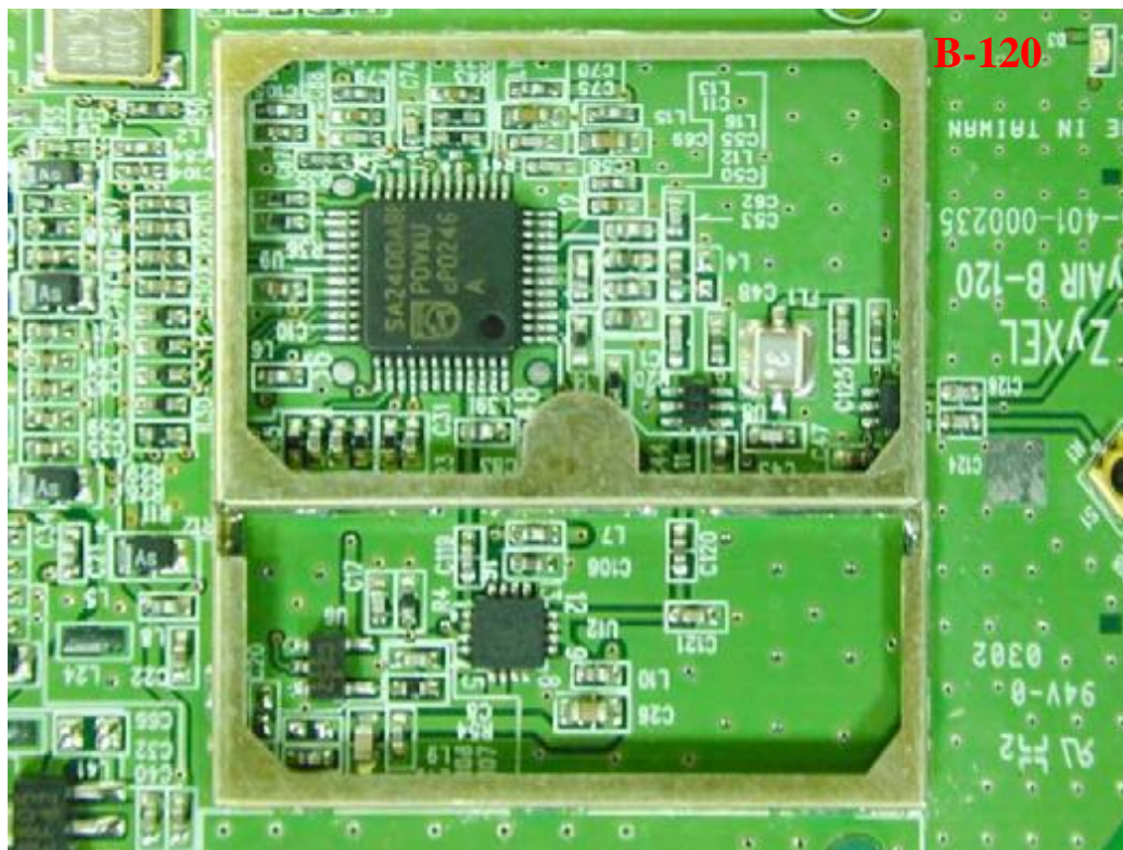
Photo 7: Interior photo of EUT
