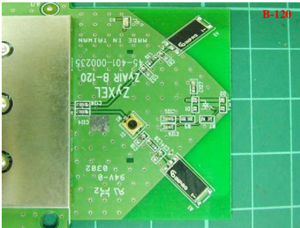
Photo 5: Interior photo of EUT
