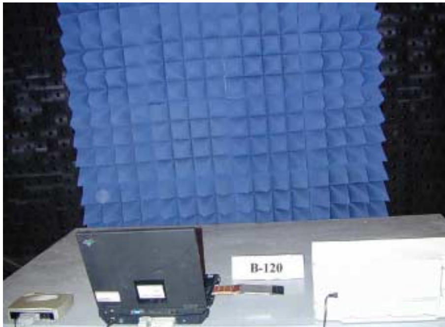
Photo 2: Spurious Test Set-up (rear)
